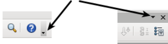
Figure 6: Customizing toolbars
