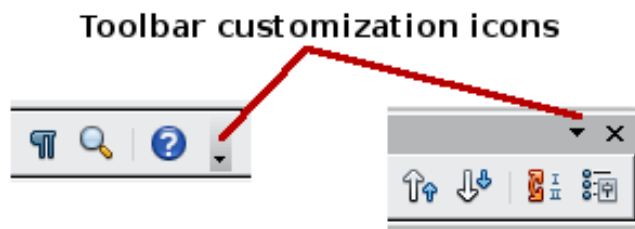
Figure 5: Customizing toolbars
