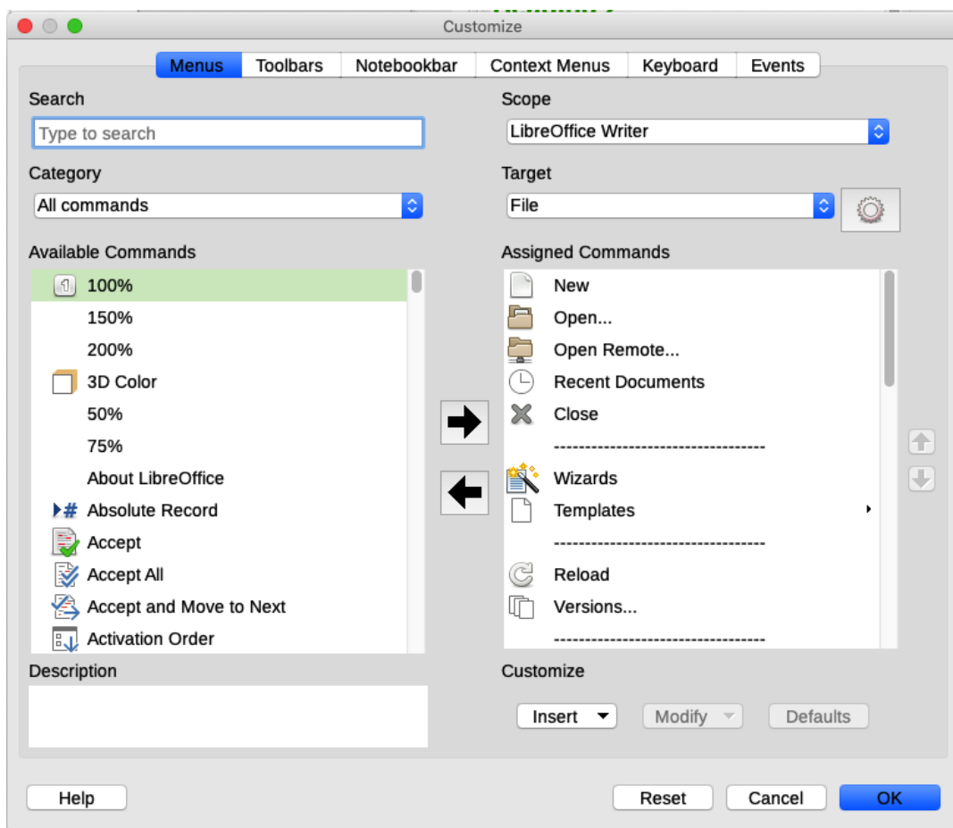
Figure 20: The Menus tab of the Customize dialog
