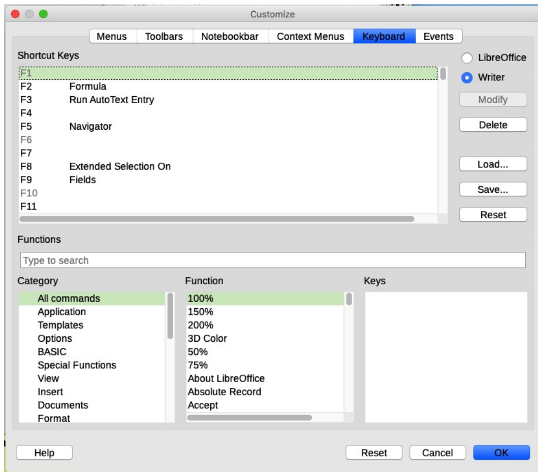
Figure 28: Defining keyboard shortcuts for applying styles
