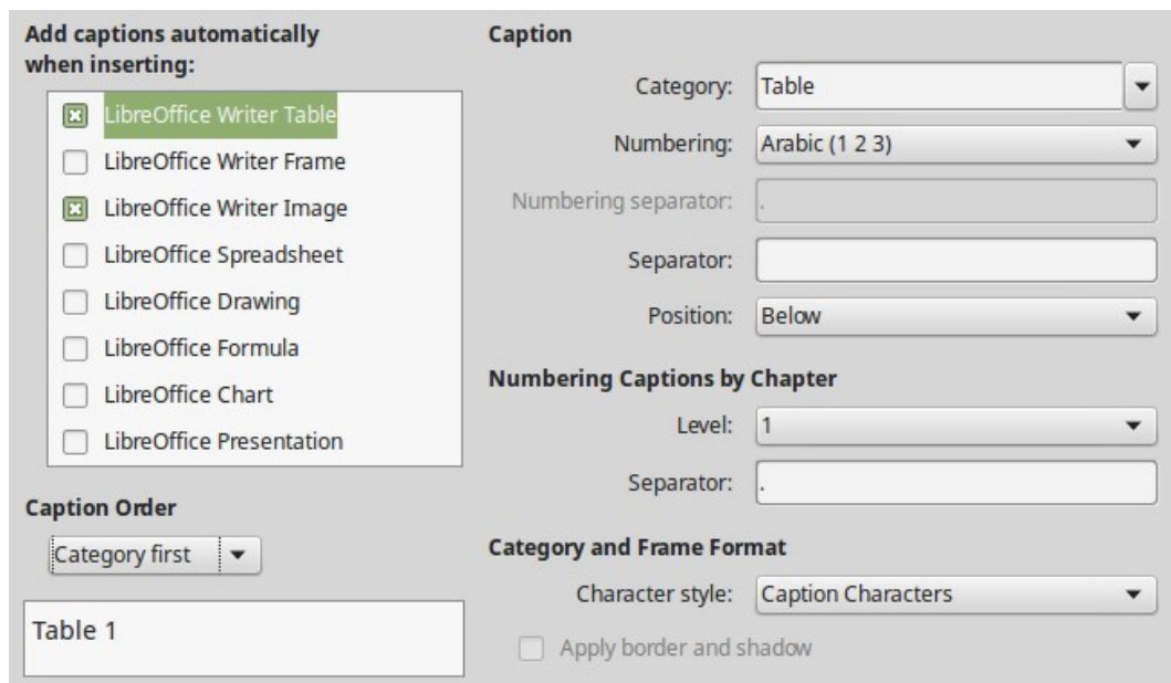
Figure 14: Setting up automatic captions
