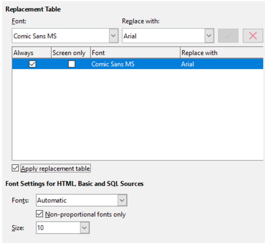
Figure 8: Defining a font to be substituted for another font
