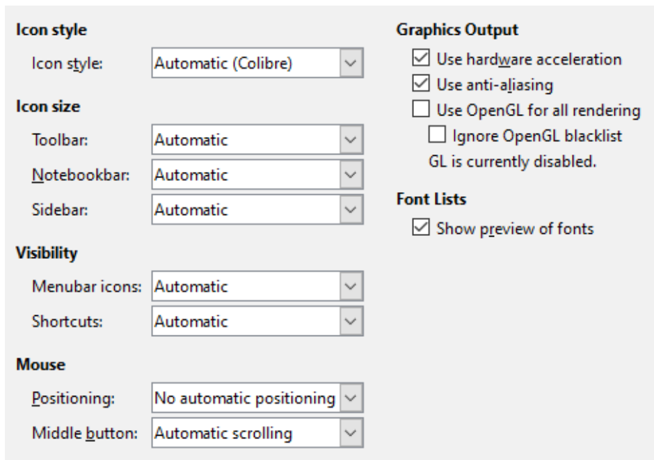
Figure 4: Choosing View options for LibreOffice applications
