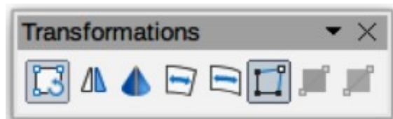
Figure 11: Transformations toolbar
