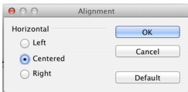
Figure 24: Alignment dialog
