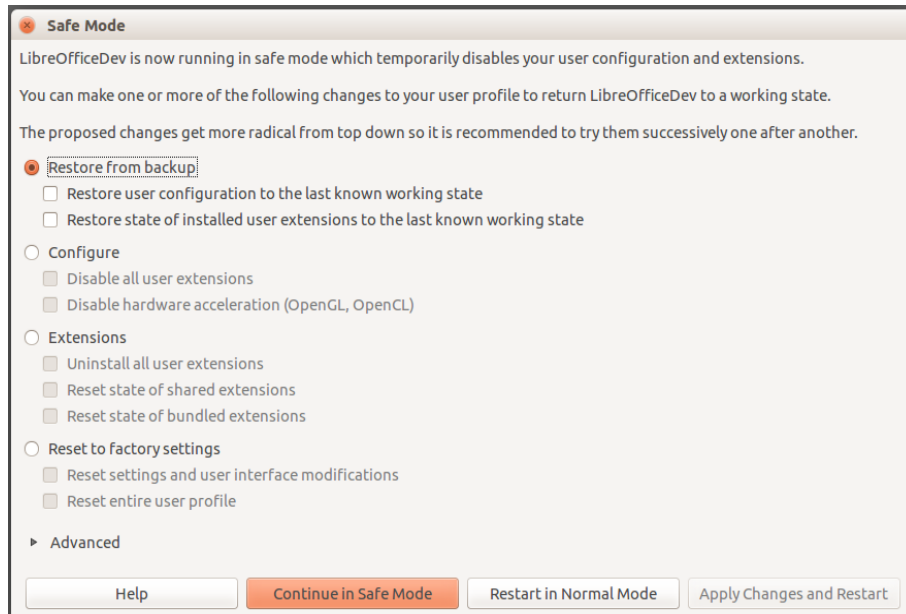
Figure 30: LibreOffice Safe Mode
