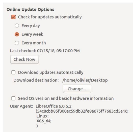
Figure 18: Online update options
