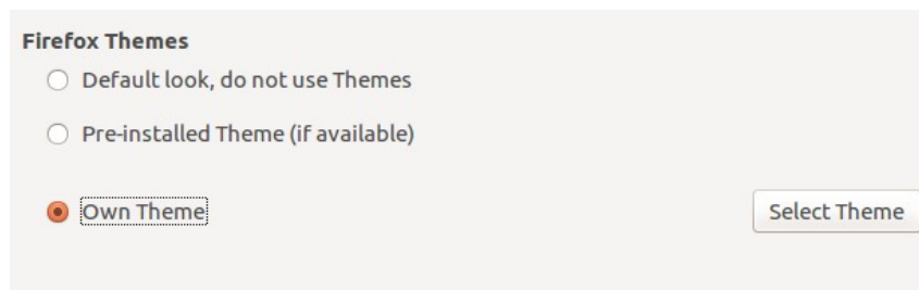
Figure 11: Personalization dialogs
