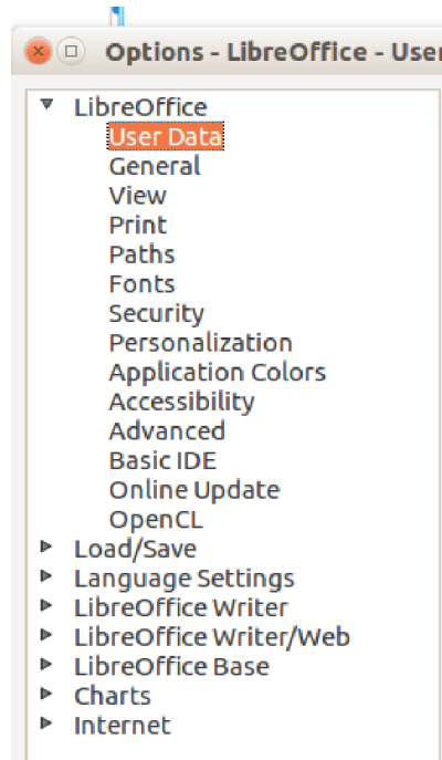
Figure 1: LibreOffice options
