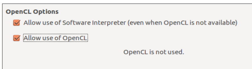
Figure 19: OpenCL options
