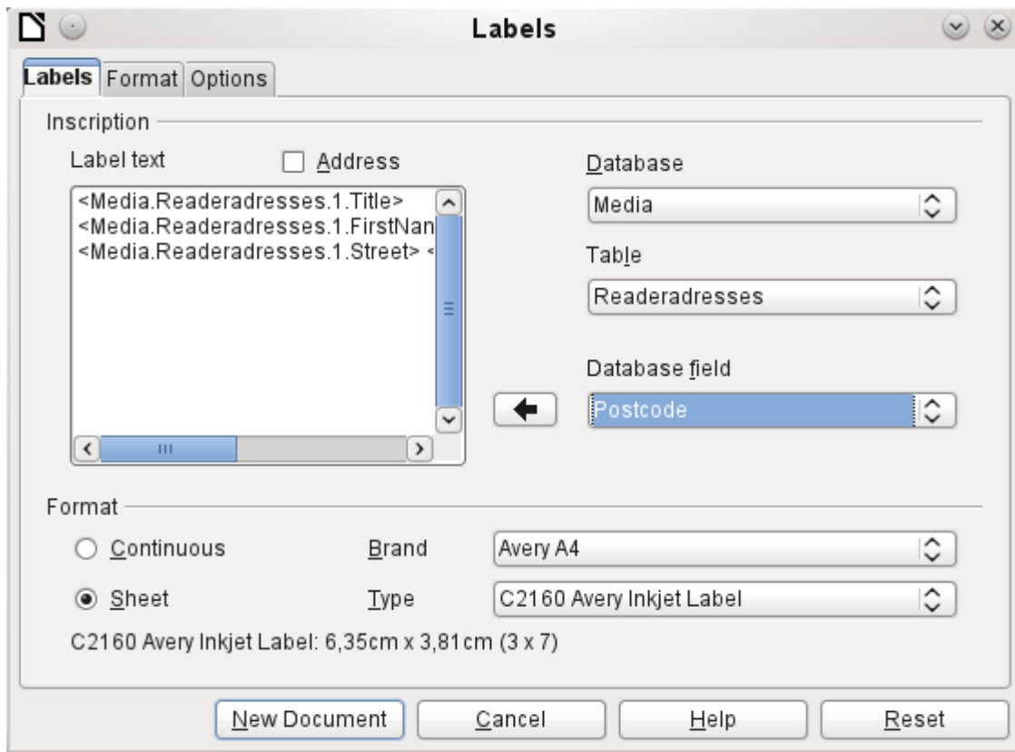
Figure 99: Labels tab of Labels dialog
