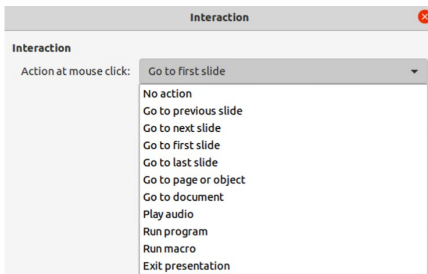
Figure 46: Interaction dialog
