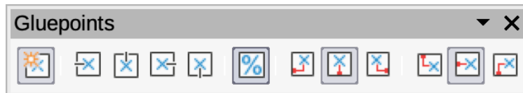
Figure 43: Gluepoints toolbar
