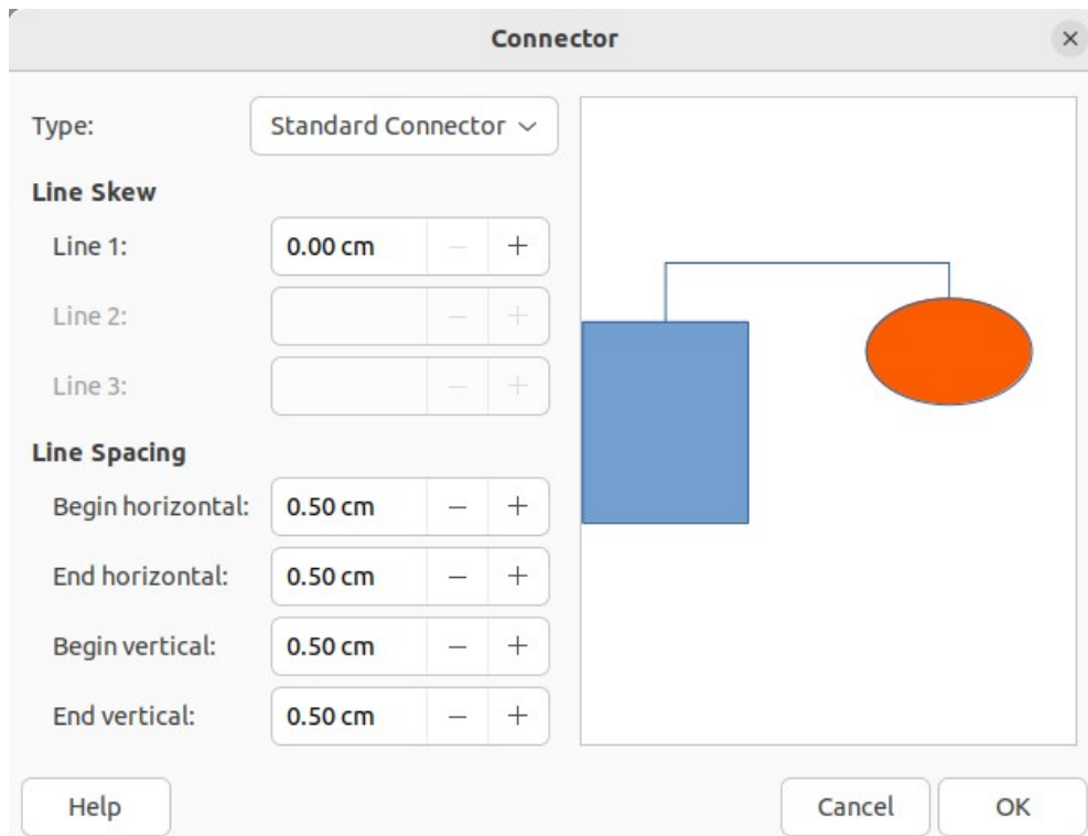
Figure 42: Connector dialog
