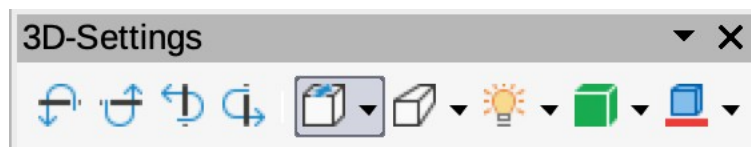
Figure 45: 3D-Settings toolbar
