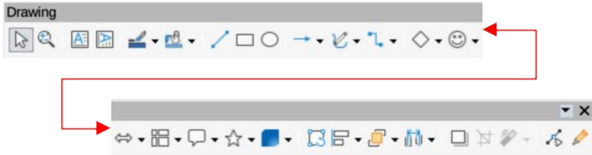
Figure 1: Drawing toolbar
