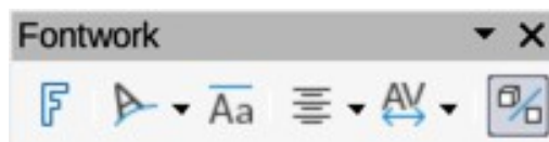
Figure 49: Fontwork toolbar
