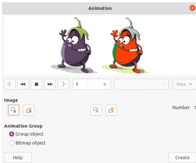
Figure 56: Animation dialog
