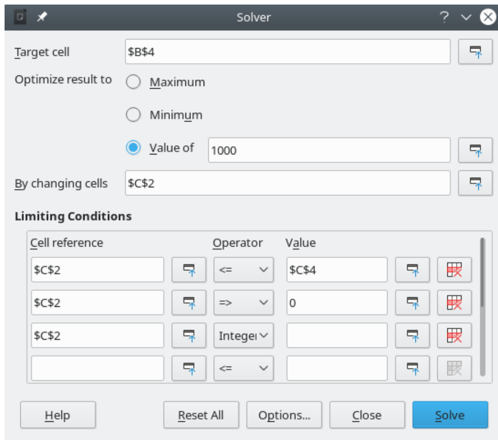
Figure 332: Solver dialog
