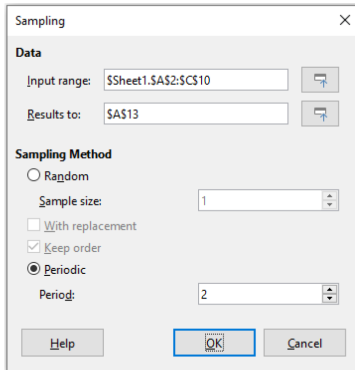
Figure 338: Sampling dialog
