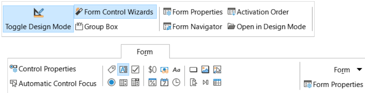
Figure 541: Form tab
