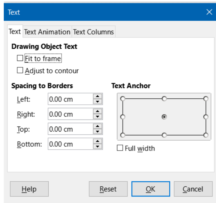
Figure 189: Text dialog
