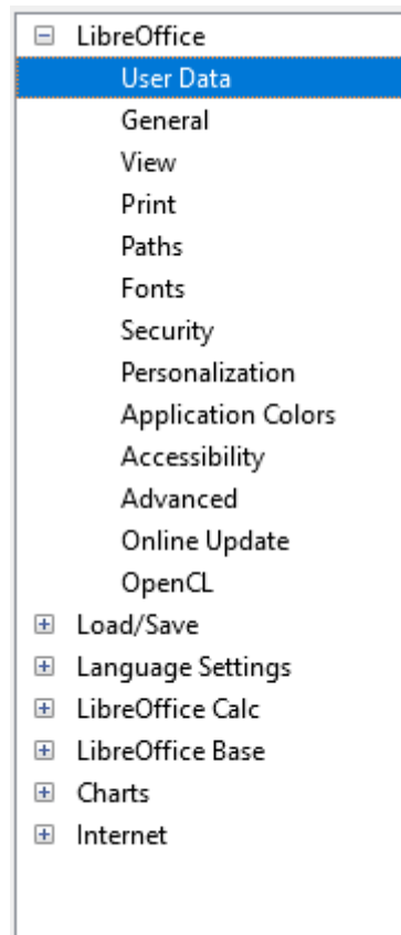
Figure 476: LibreOffice options
