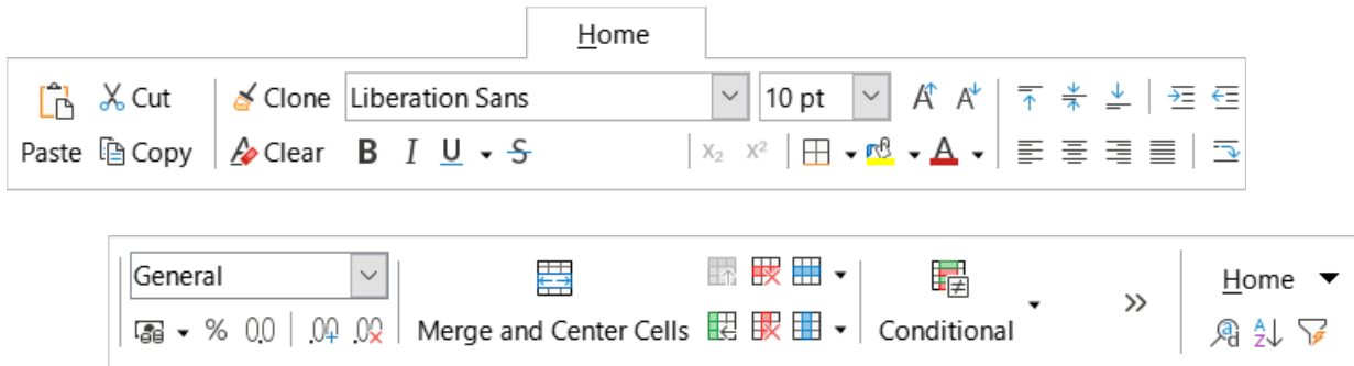
Figure 516: Home tab
