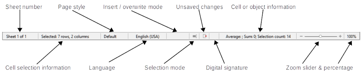
Figure 6: Status Bar
