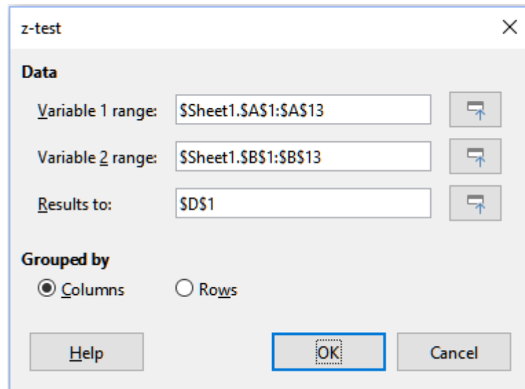
Figure 362: z-test dialog
