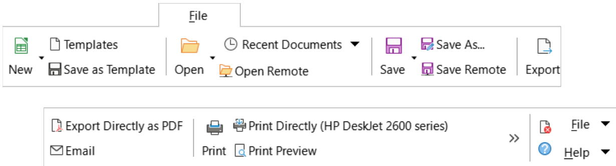
Figure 513: File tab
