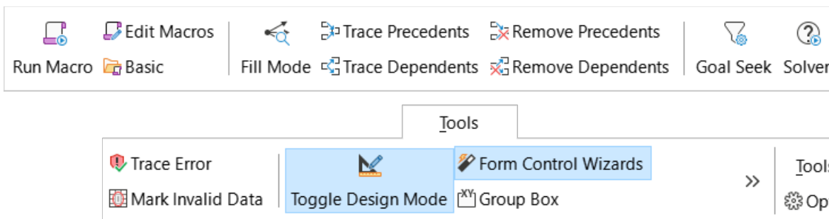
Figure 535: Tools tab
