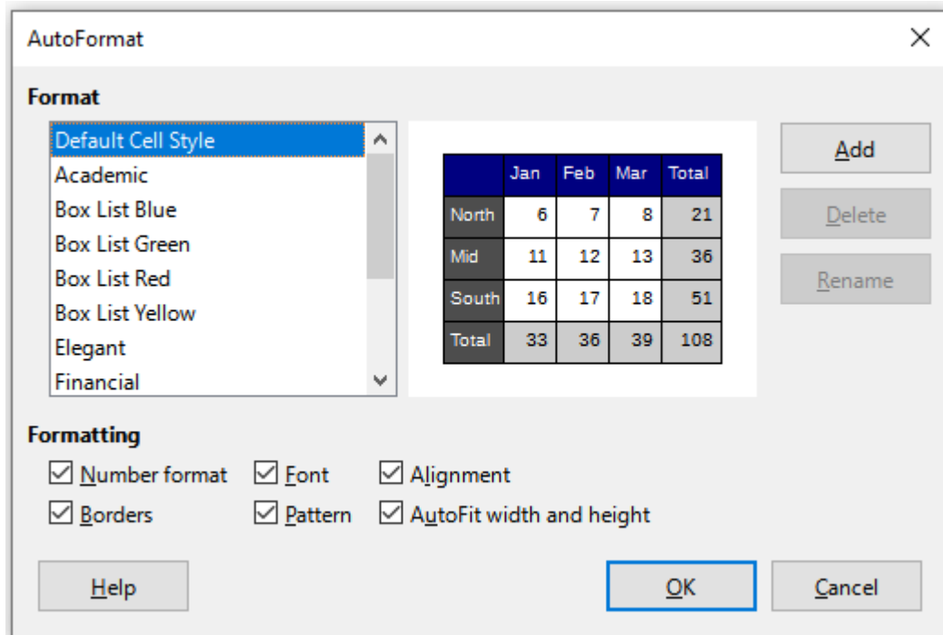
Figure 52: AutoFormat dialog
