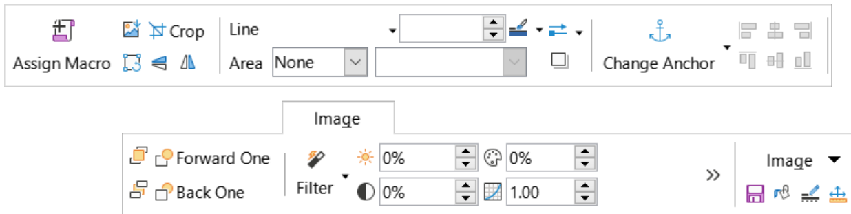
Figure 543: Image tab
