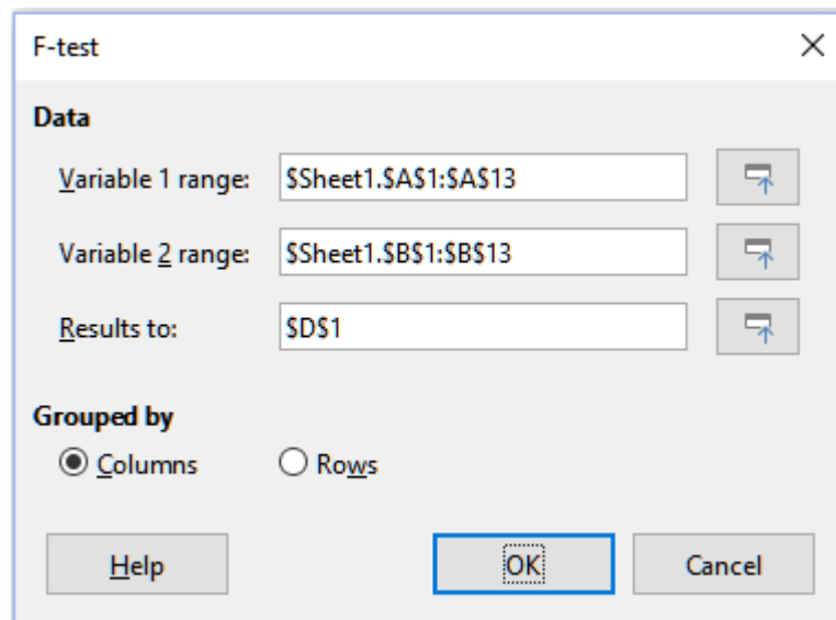
Figure 360: F-test dialog
