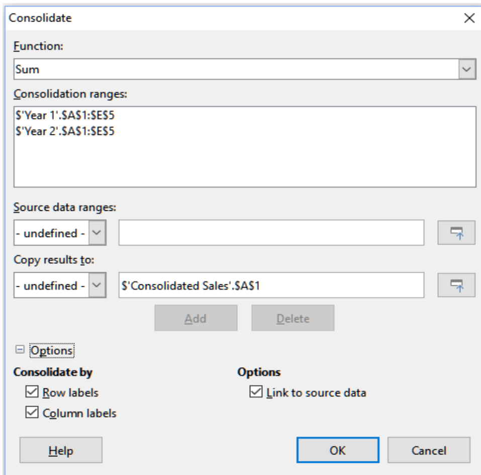
Figure 305: Consolidate dialog
