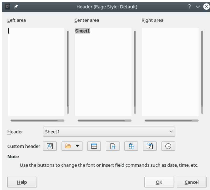
Figure 213: Header dialog
