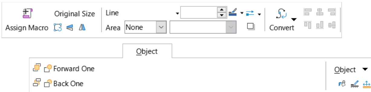
Figure 548: Object tab
