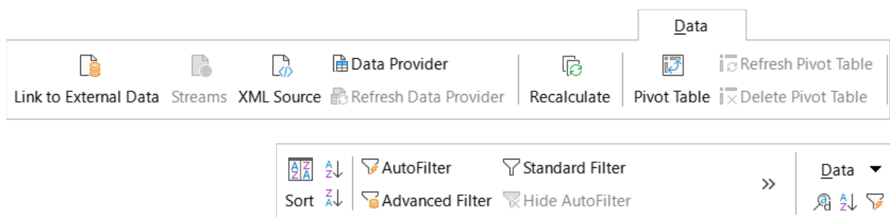
Figure 525: Data tab
