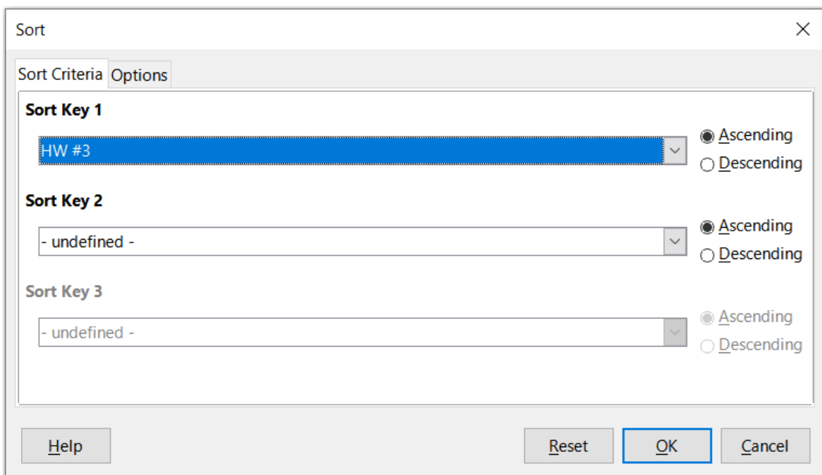
Figure 469: Sort dialog
