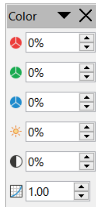
Figure 187: Color toolbar
