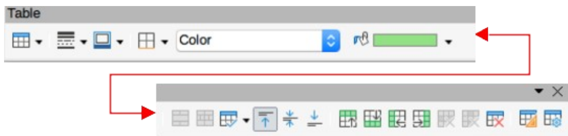
Figure 35: Table toolbar
