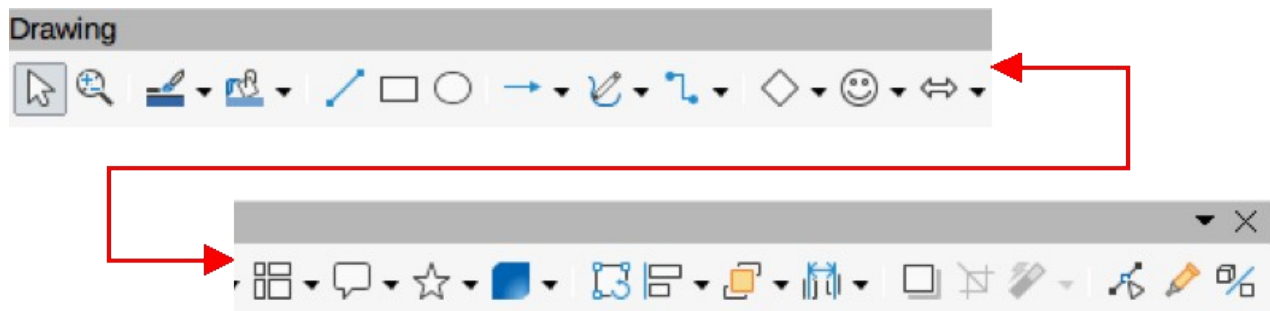
Figure 2: Drawing toolbar
