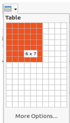
Figure 37: Table graphic
