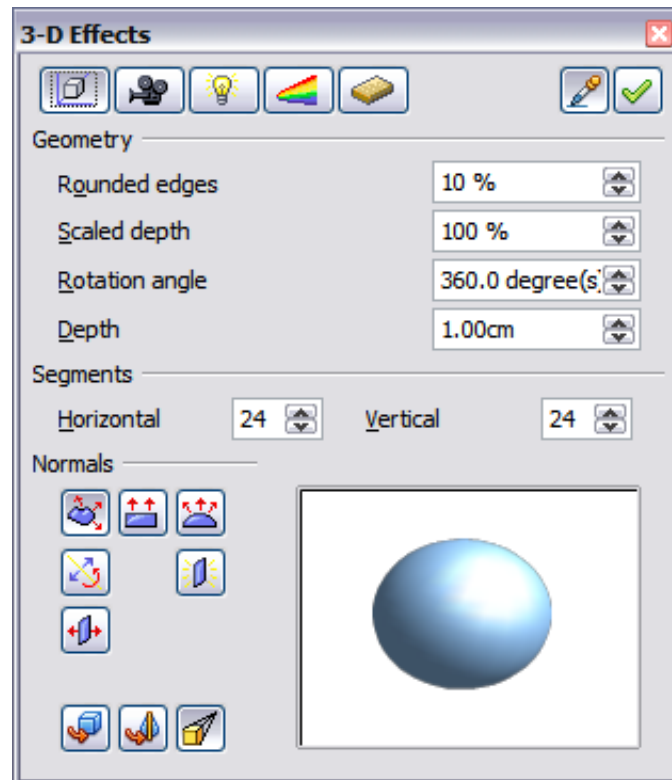
Figure 14: Geometry page
