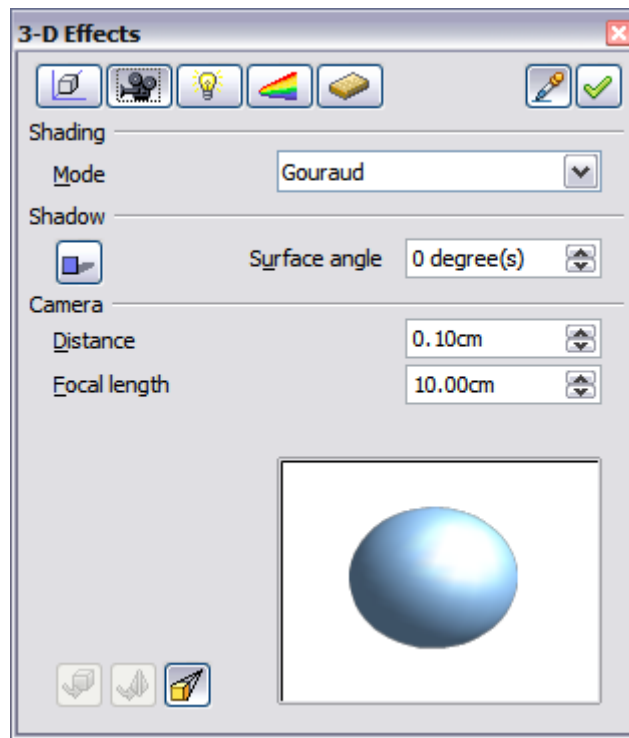
Figure 24: Shading page
