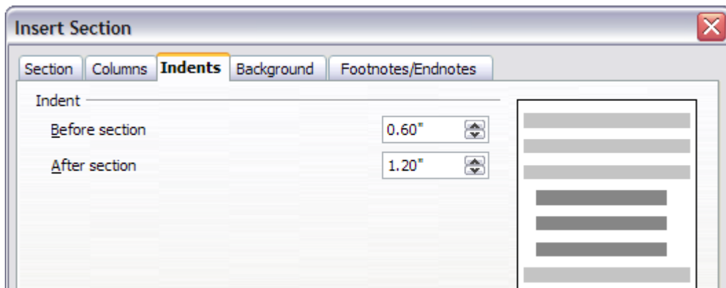
Figure 30: Indenting sections
