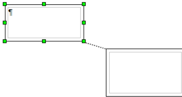
Figure 17: Linked frames
