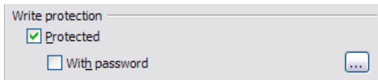
Figure 27: Write-protecting sections
