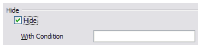
Figure 29: Hiding sections
