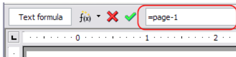
Figure 50: Formula bar
