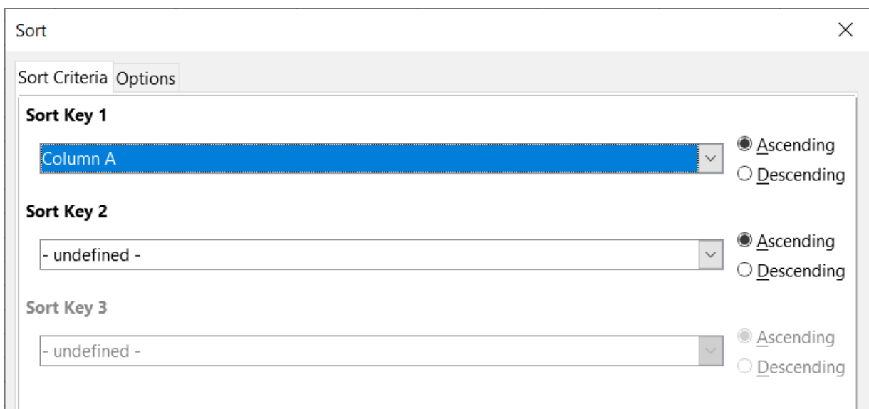
Figure 10: Sort dialog
