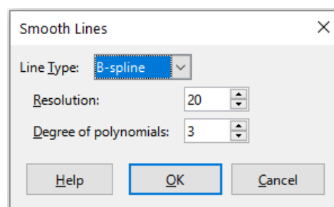
Figure 67: Smooth Lines dialog
