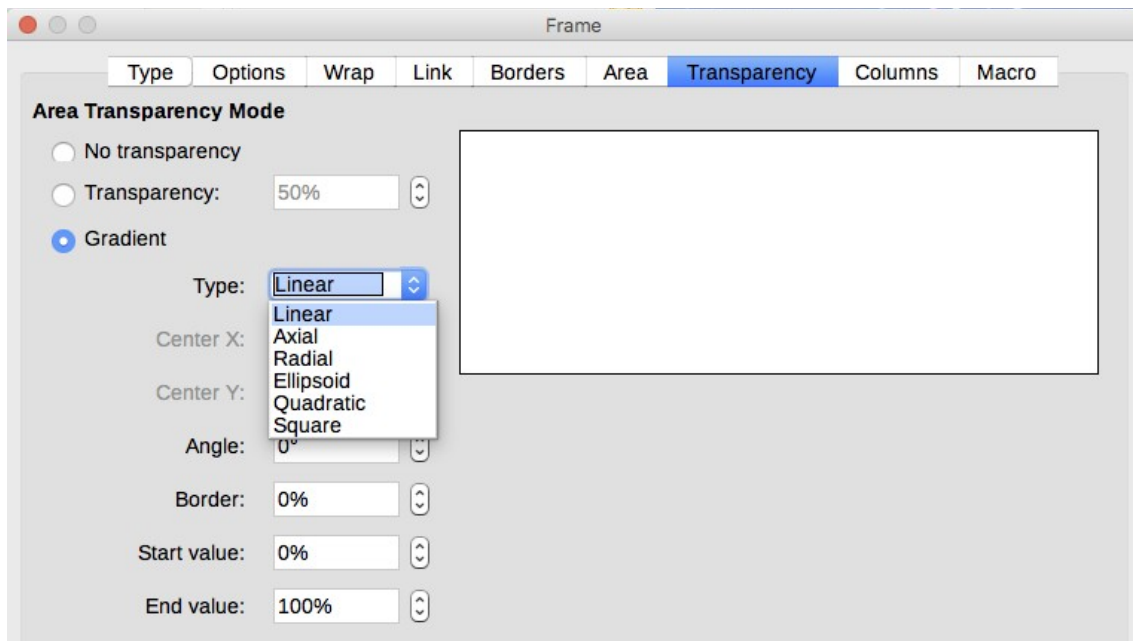
Figure 144: Transparency options
