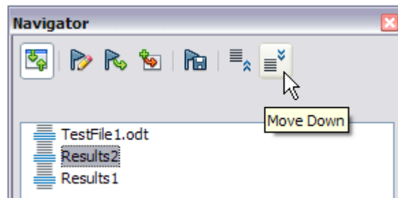
Figure 373: Moving subdocuments
