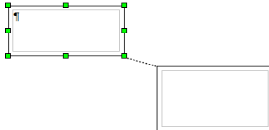
Figure 116: Linked frames
