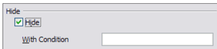
Figure 126: Hiding sections
