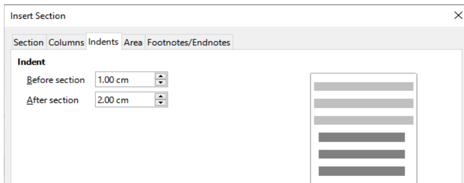
Figure 129: Indenting sections
