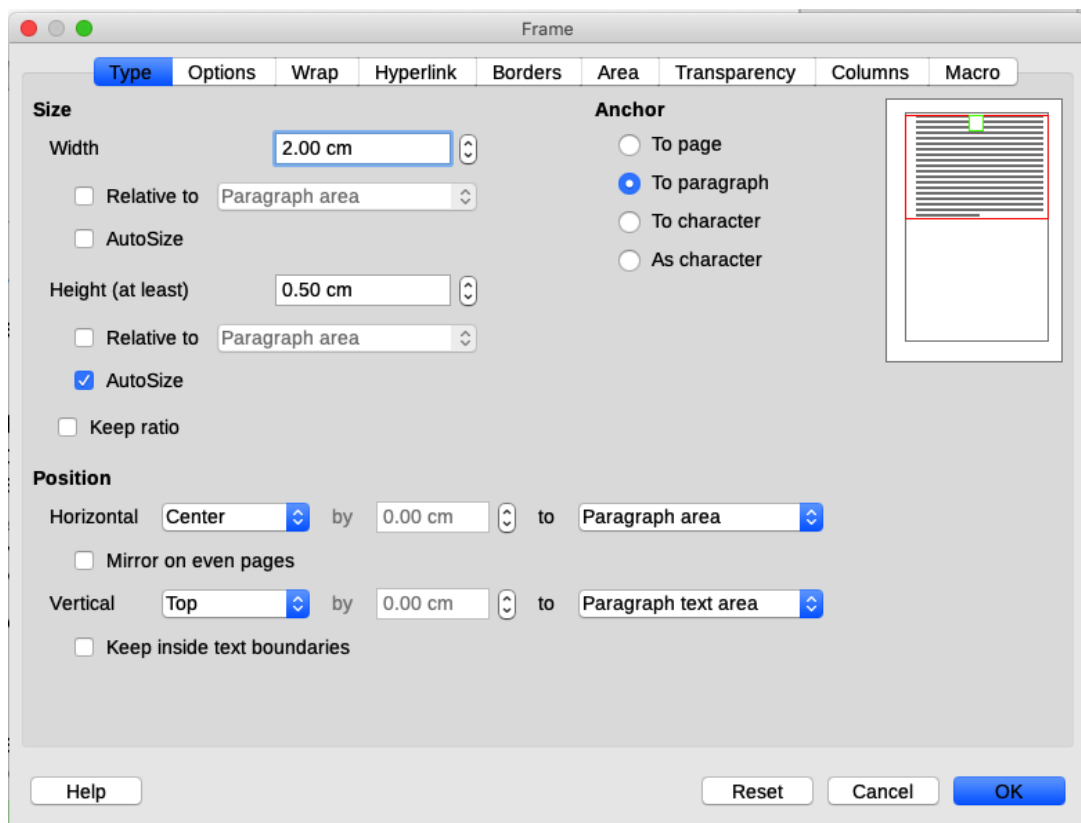
Figure 113: Frame dialog
