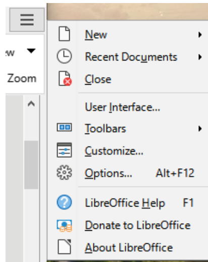
Figure 471: Quick menu
