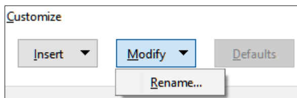
Figure 456: Modify drop-down
