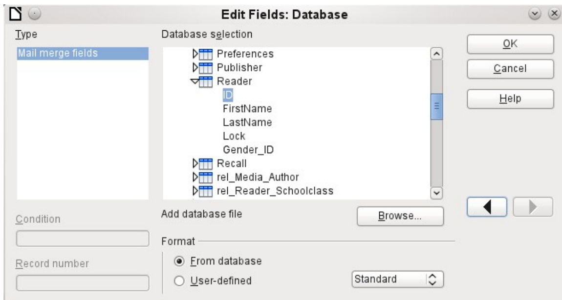
Figure 8: Double-click on an inserted field to show the properties of the Mail Merge fields
