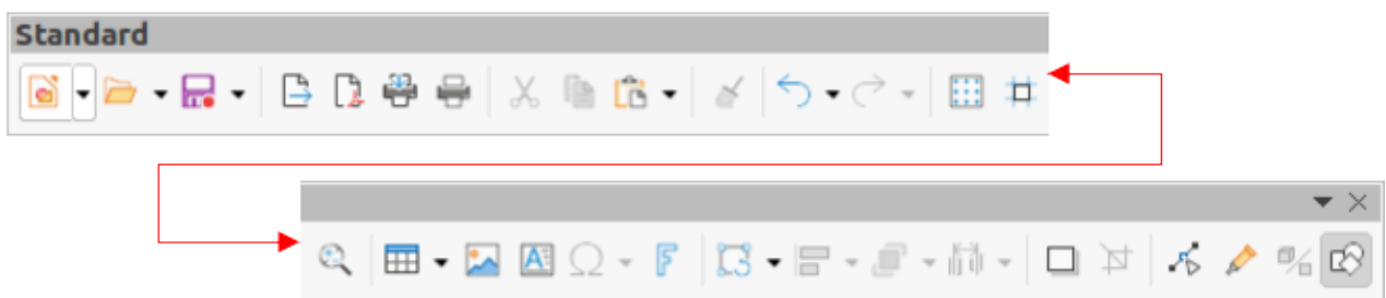
Figure 200: Standard toolbar
