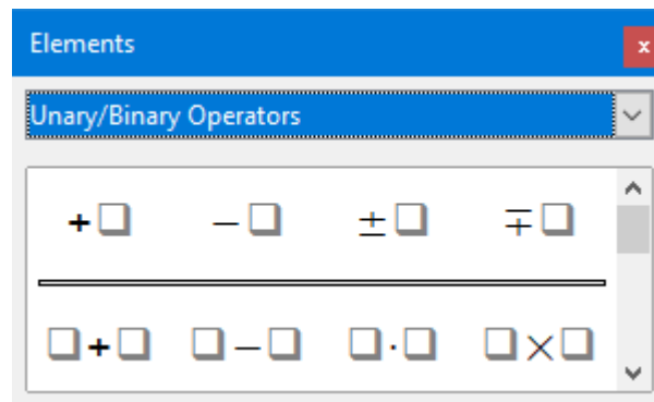
Figure 324: Elements dialog
