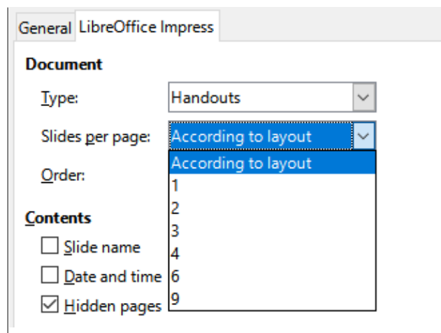
Figure 19: Handouts
