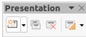
Figure 158: Presentation toolbar
