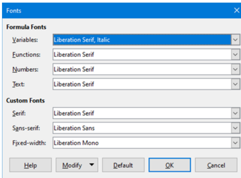
Figure 315: Fonts dialog
