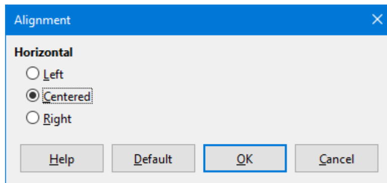
Figure 317: Alignment dialog
