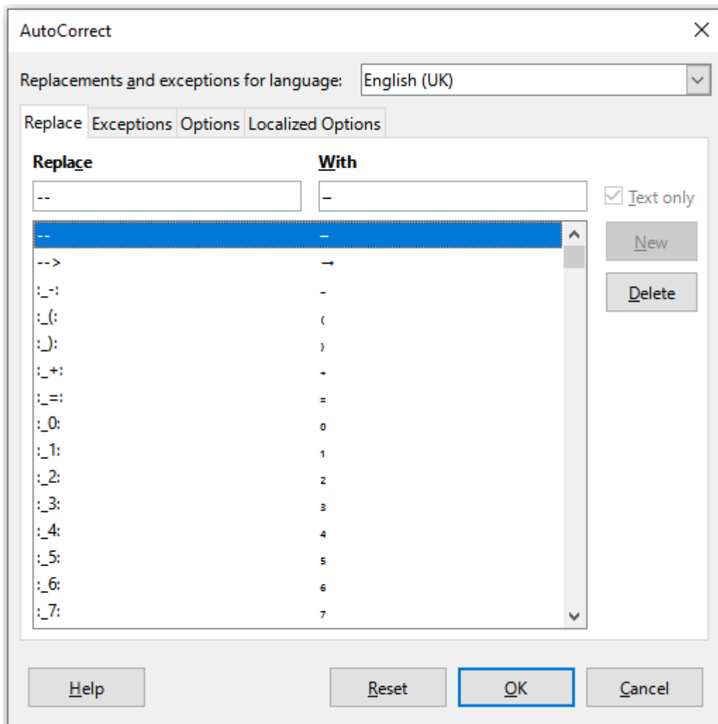
Figure 84: AutoCorrect dialog
