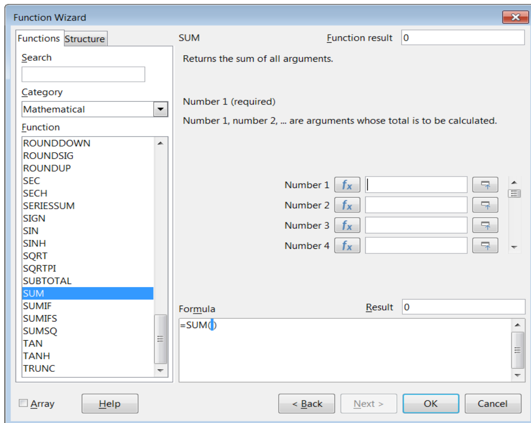
Figure 99: Function Wizard
