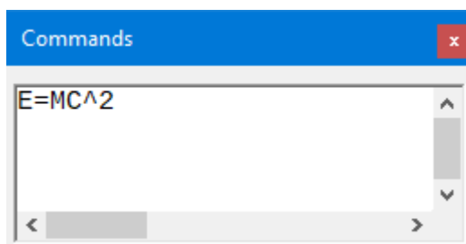
Figure 323: Commands dialog
