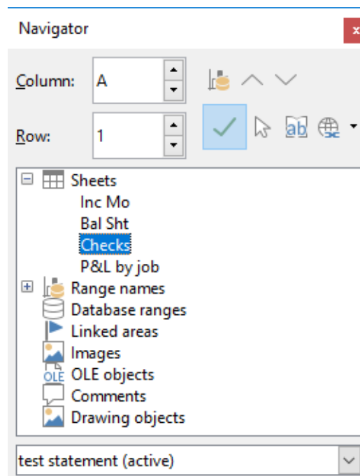
Figure 71: Calc Navigator
