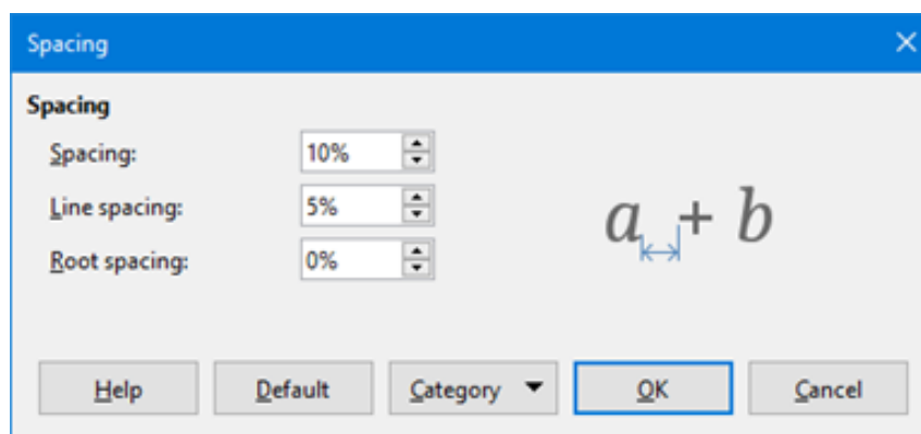
Figure 316: Spacing dialog
