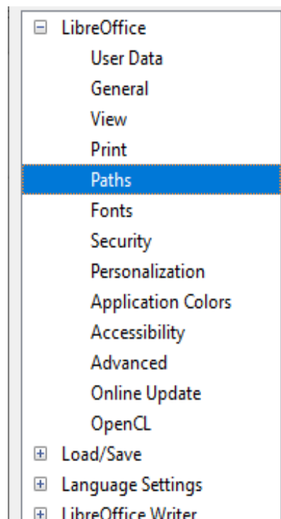
Figure 377: LibreOffice options
