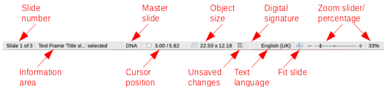
Figure 151: Status bar
