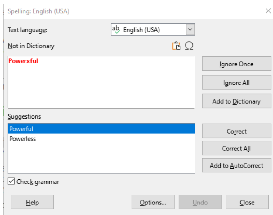
Figure 42: Spelling dialog
