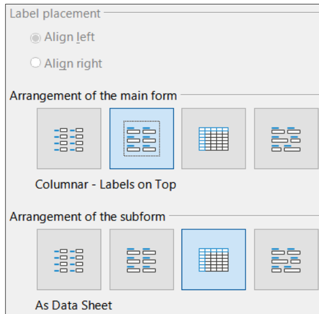
Figure 263: Arrange controls
