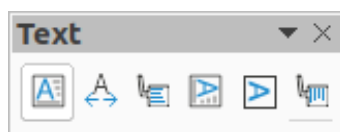
Figure 161: Text toolbar
