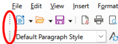
Figure 4: Toolbar handles
