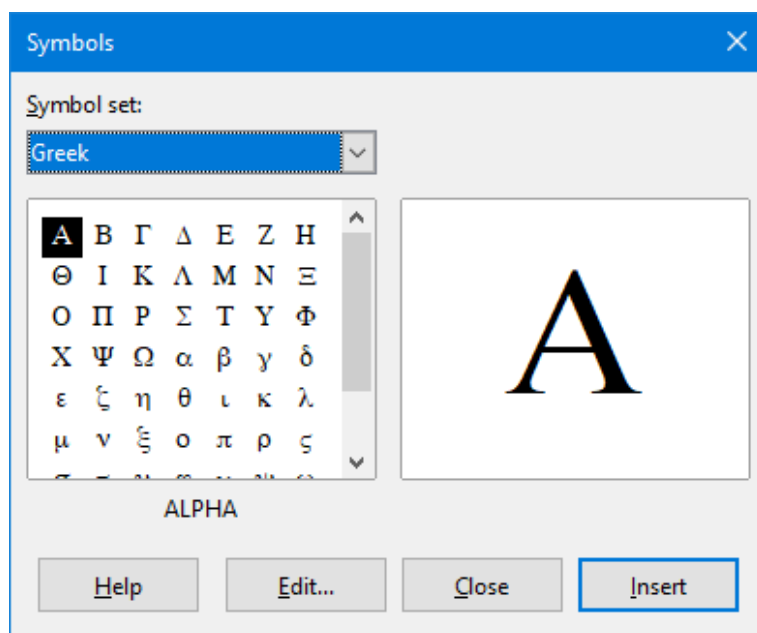
Figure 312: Symbols dialog
