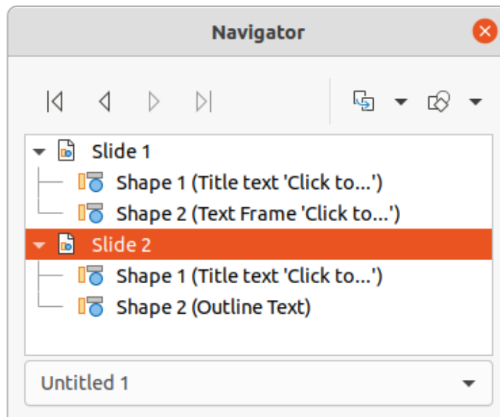
Figure 152: Navigator dialog
