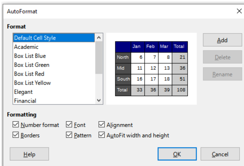
Figure 93: AutoFormat dialog
