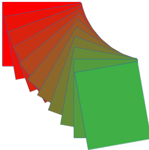
Figure 234: Duplication example
