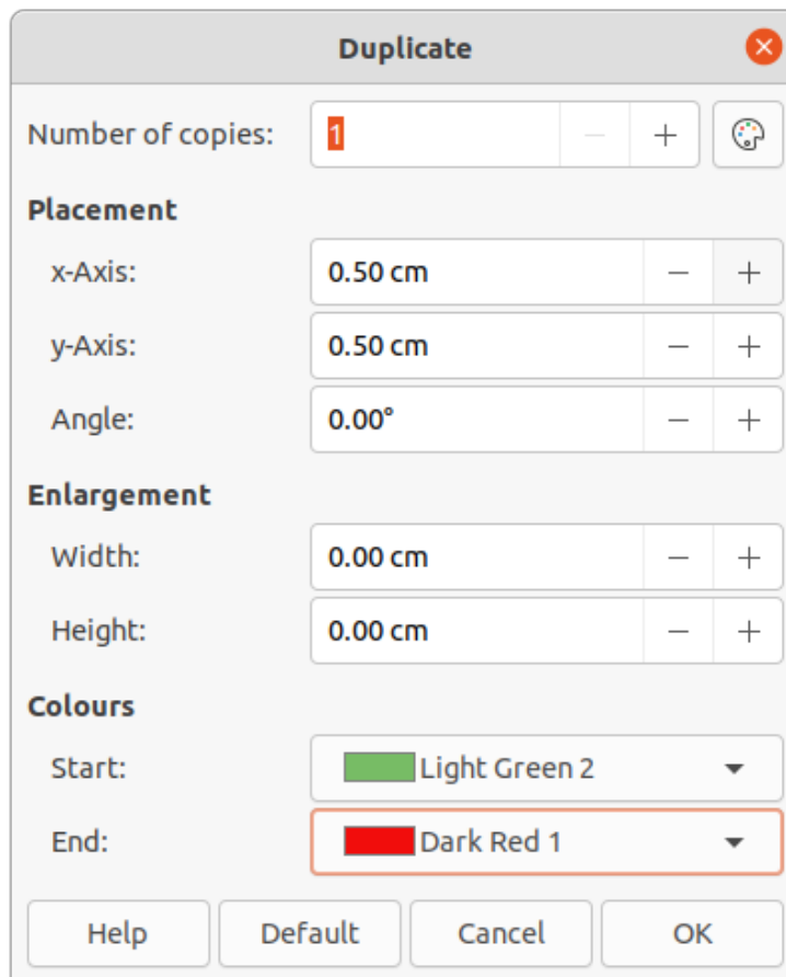
Figure 235: Duplicate dialog
