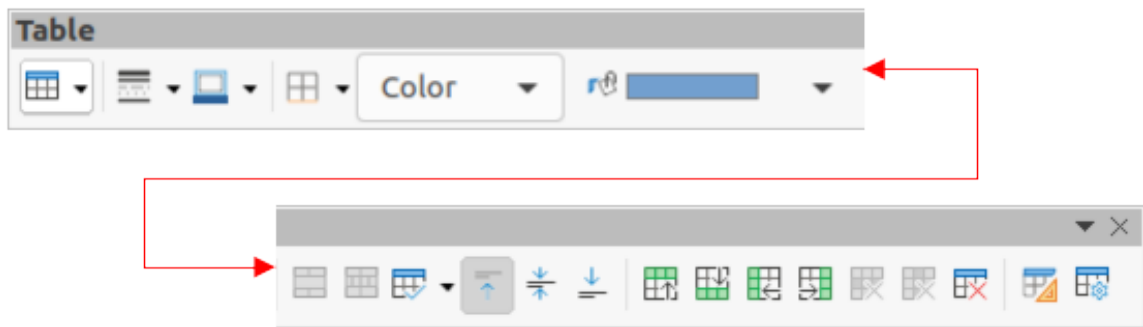
Figure 169: Table toolbar
