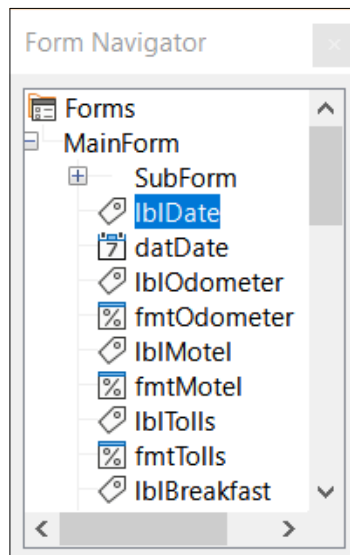
Figure 266: Form Navigator
