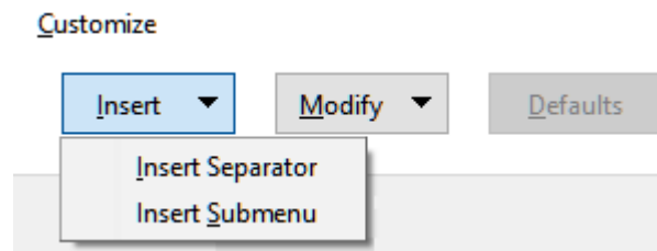
Figure 402: Insert drop-down
