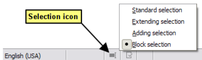
Figure 35: Selection icon
