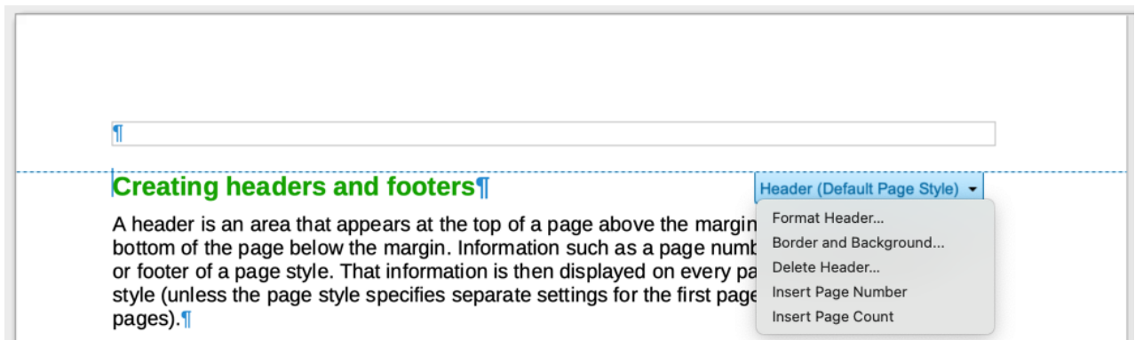
Figure 52: Header menu
