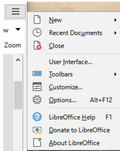
Figure 418: Quick menu
