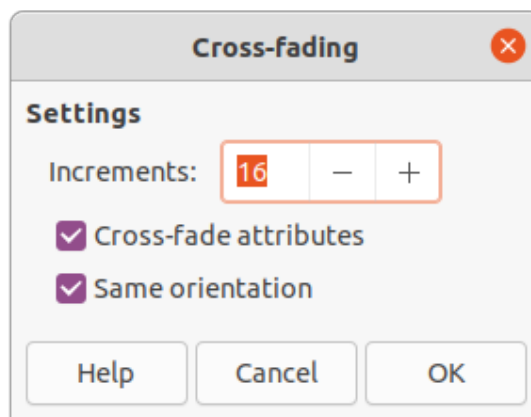
Figure 237: Cross-fading dialog
