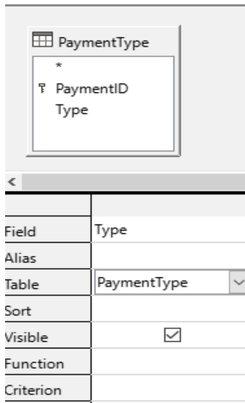
Figure 267: Selecting PaymentType
