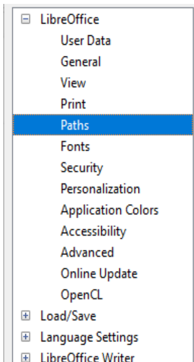
Figure 25: LibreOffice options
