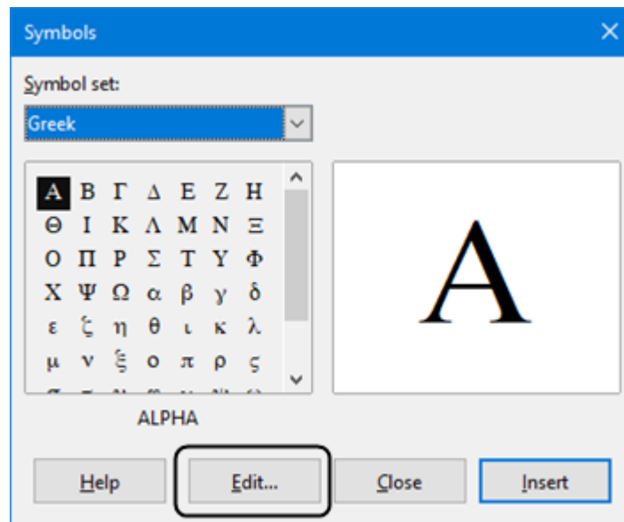
Figure 325: Symbols dialog
