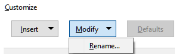
Figure 403: Modify drop-down
