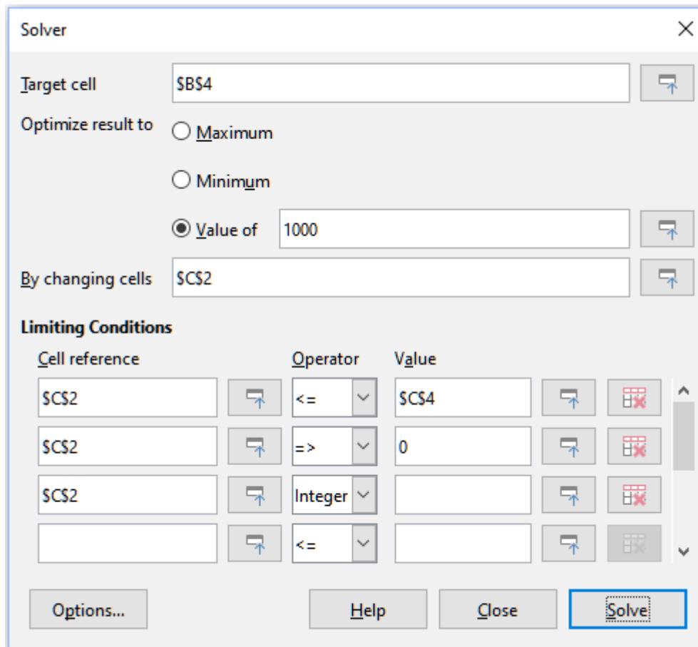
Figure 326: Solver dialog
