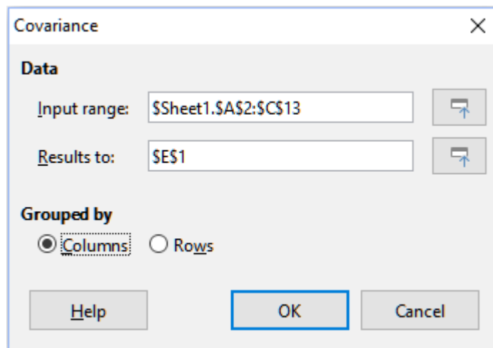
Figure 340: Covariance dialog
