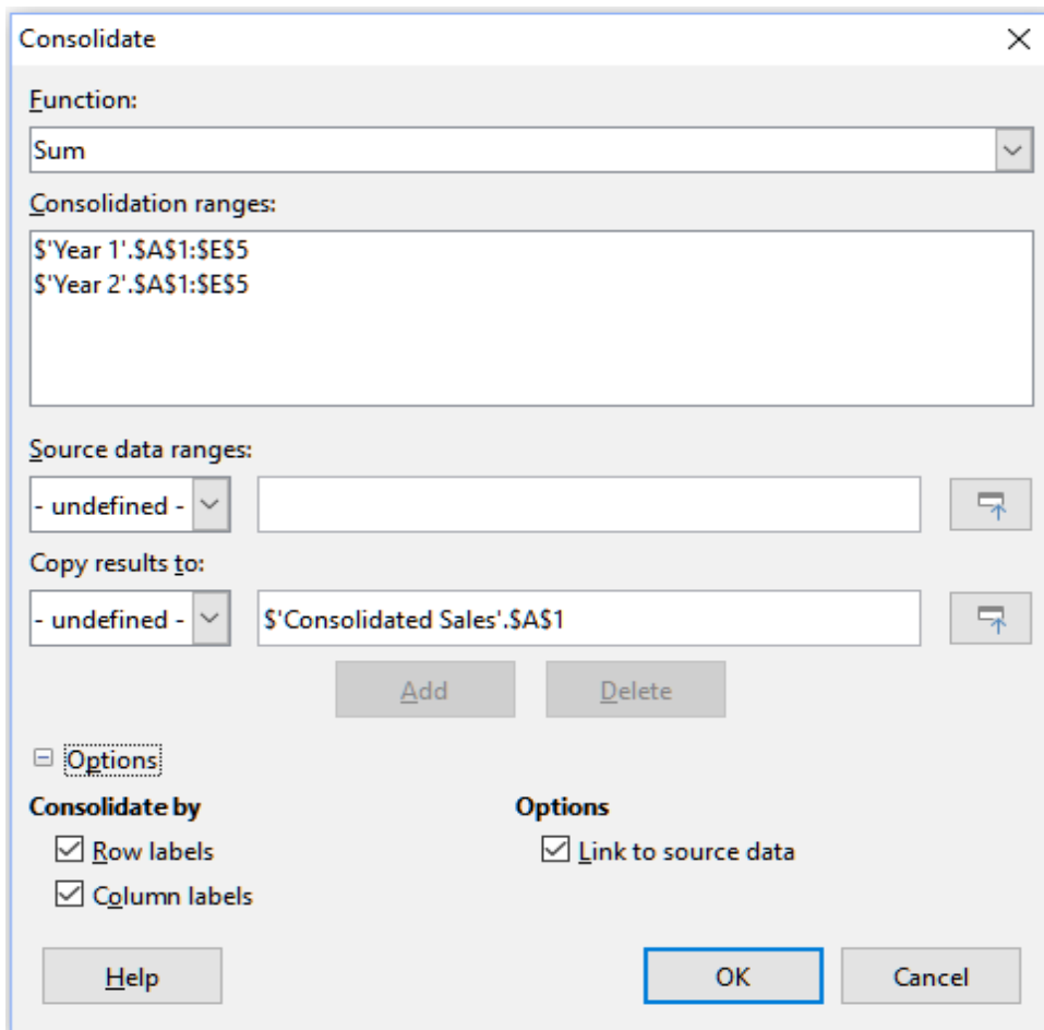
Figure 299: Consolidate dialog
