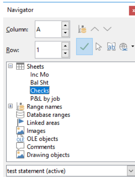
Figure 12: Navigator dialog
