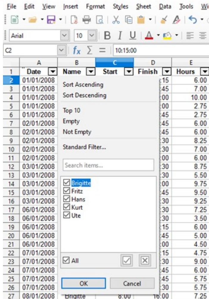
Figure 65: AutoFilter example
