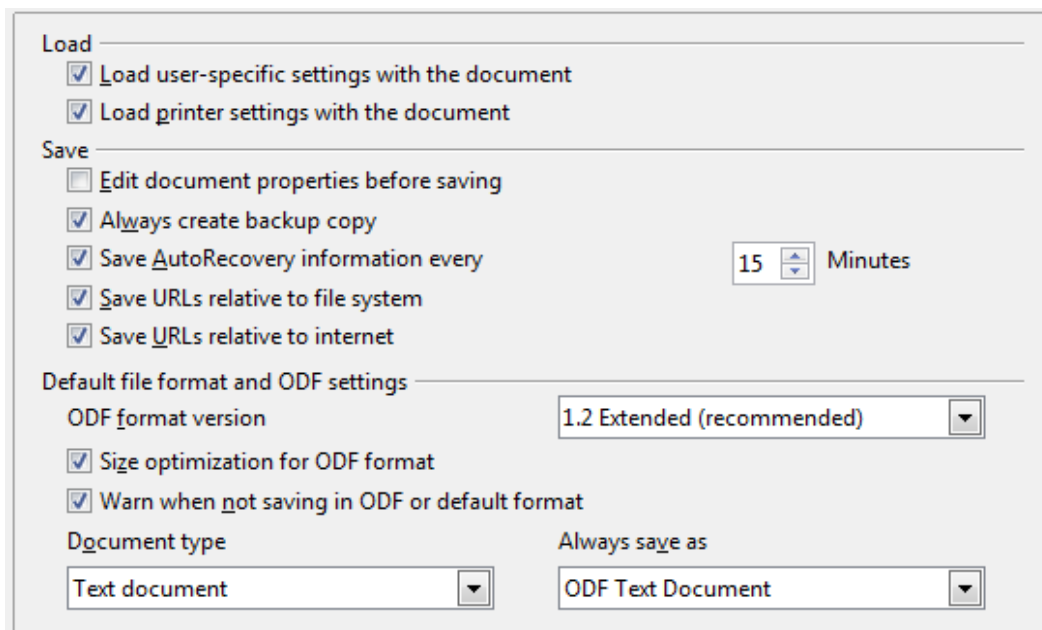
Figure 18. Choosing Load and Save options
