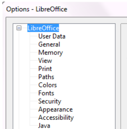
Figure 1: LibreOffice options
