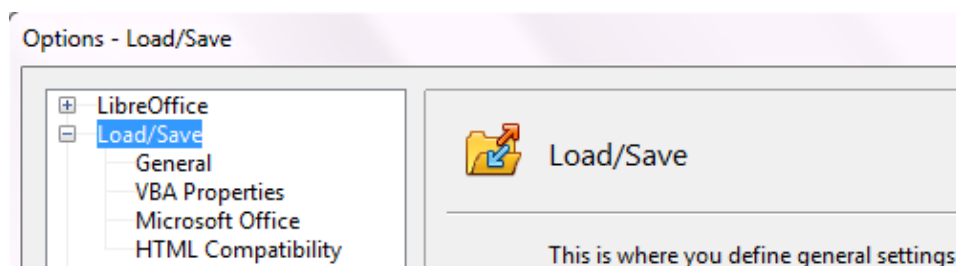
Figure 17: Load/Save options
