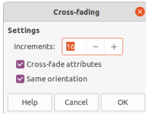
Figure 43: Cross-fading dialog
