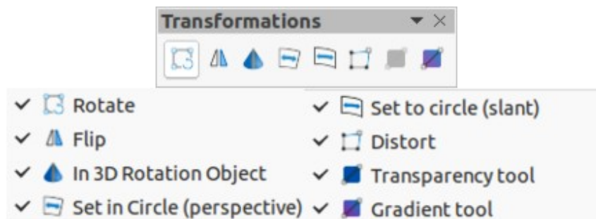
Figure 38: Transformations toolbar
