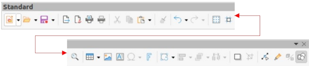
Figure 5: Standard toolbar
