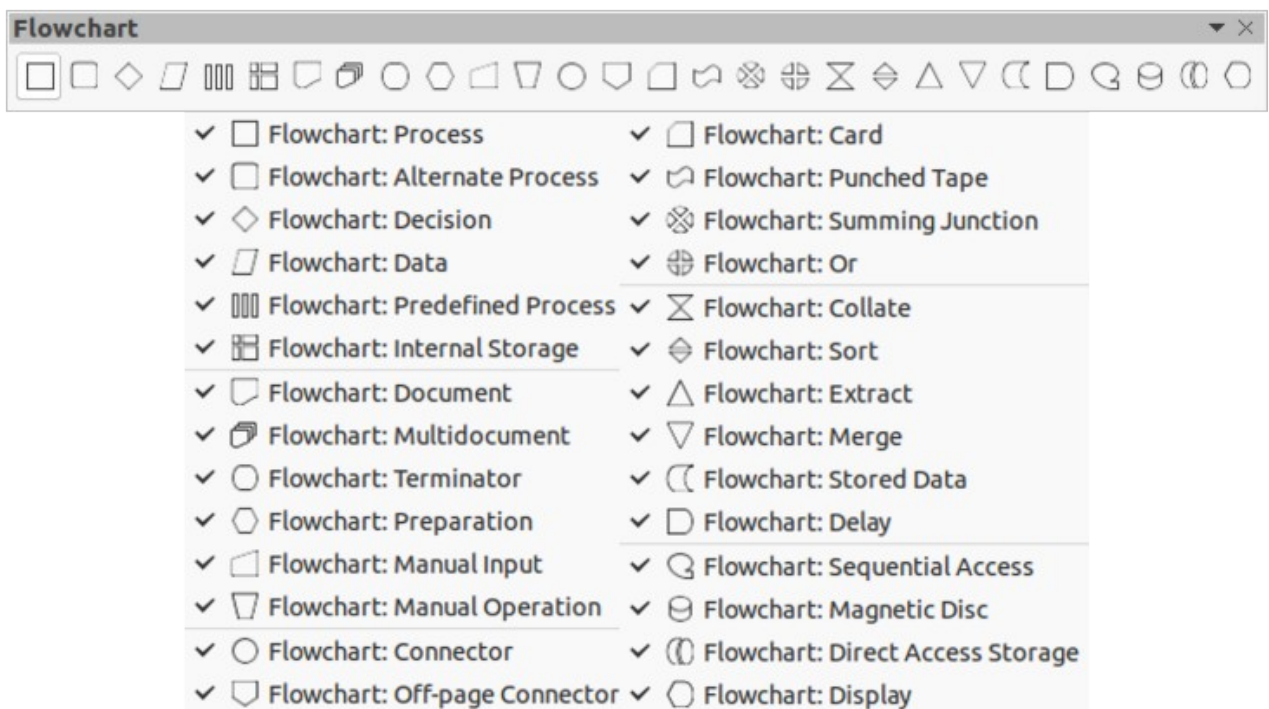
Figure 26: Flowchart sub-toolbar
