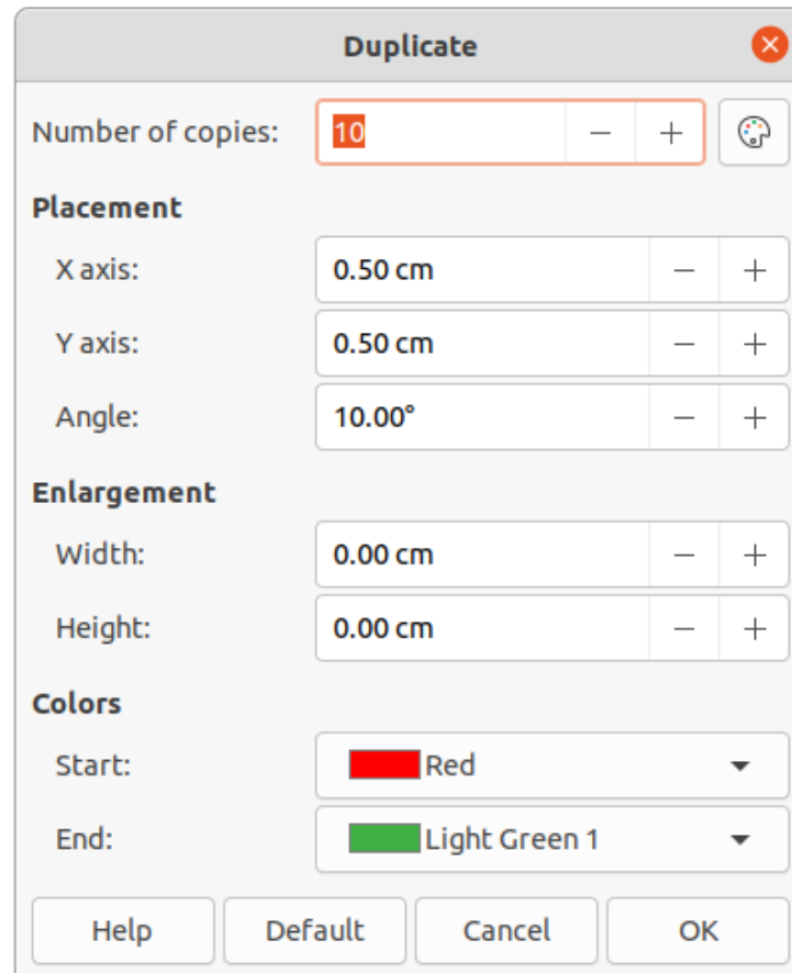
Figure 41: Duplicate dialog
