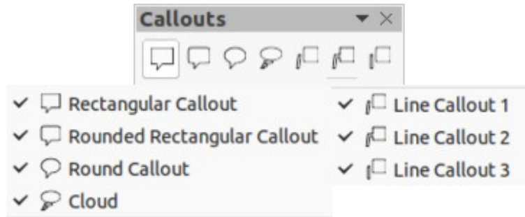
Figure 27: Callouts sub-toolbar
