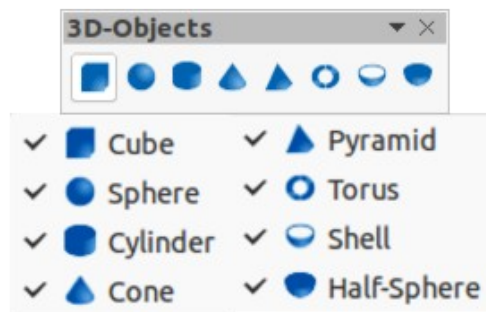
Figure 29: 3D-Objects sub-toolbar
