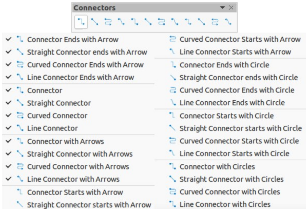
Figure 22: Connectors sub-toolbar
