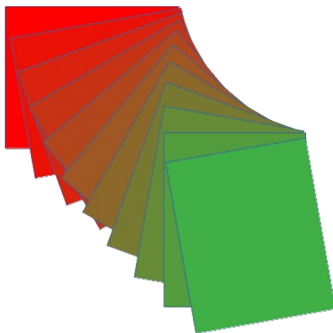
Figure 40: Duplication example
