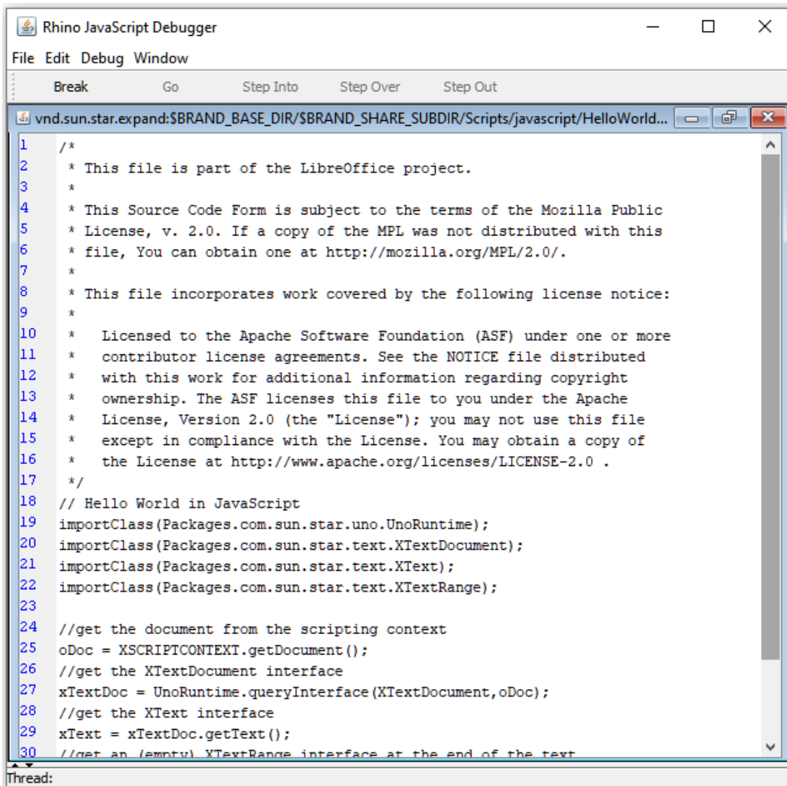
Figure 369: Rhino JavaScript Debugger
