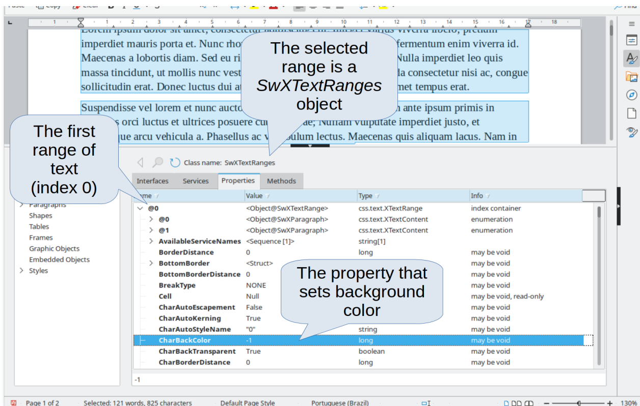
Figure 363: Using the Object Inspector to find a property
