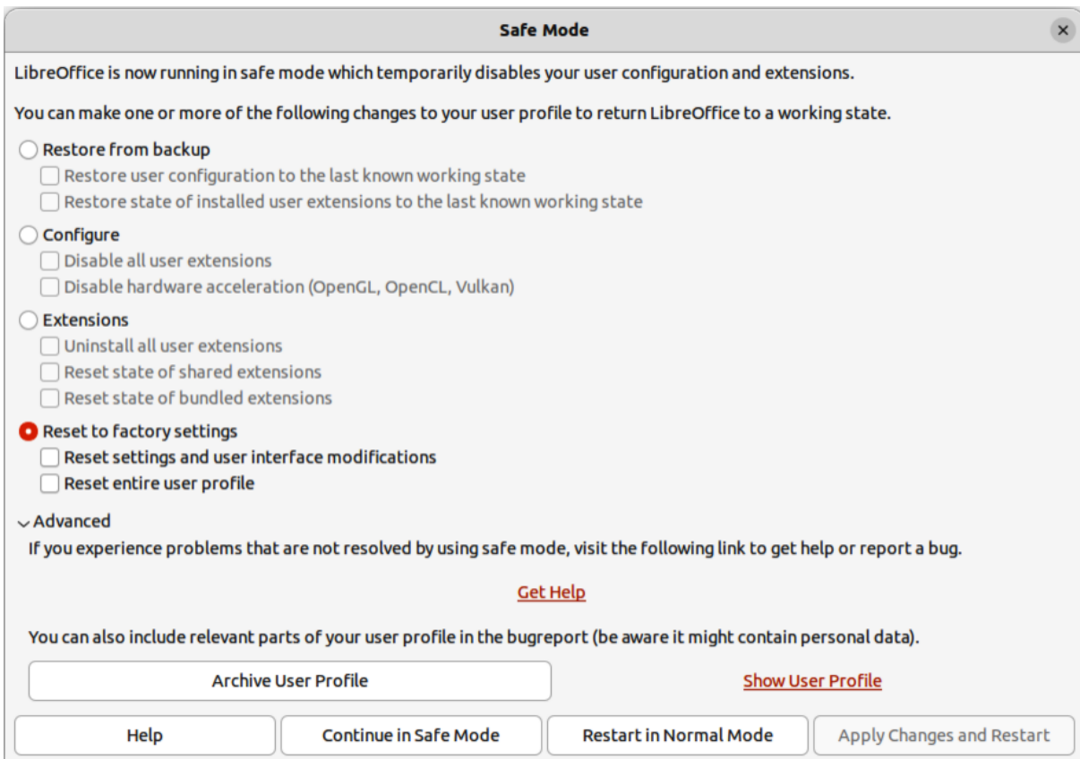
Figure 19: Safe Mode dialog
