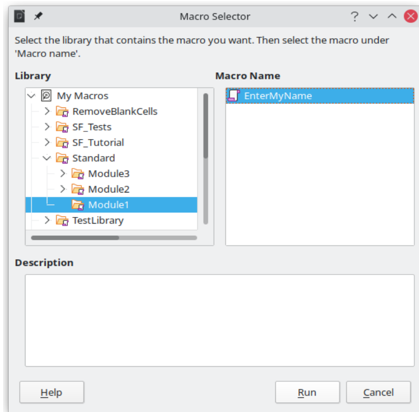
Figure 350: Use the Macro Selector dialog to select and run an existing macro
