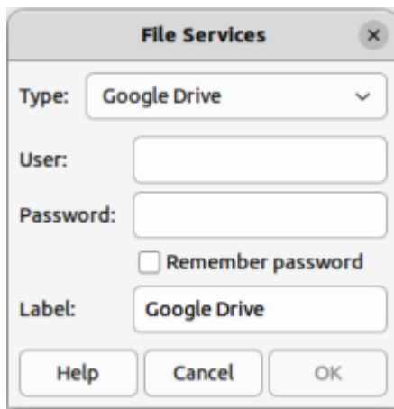
Figure 331: File Services dialog
