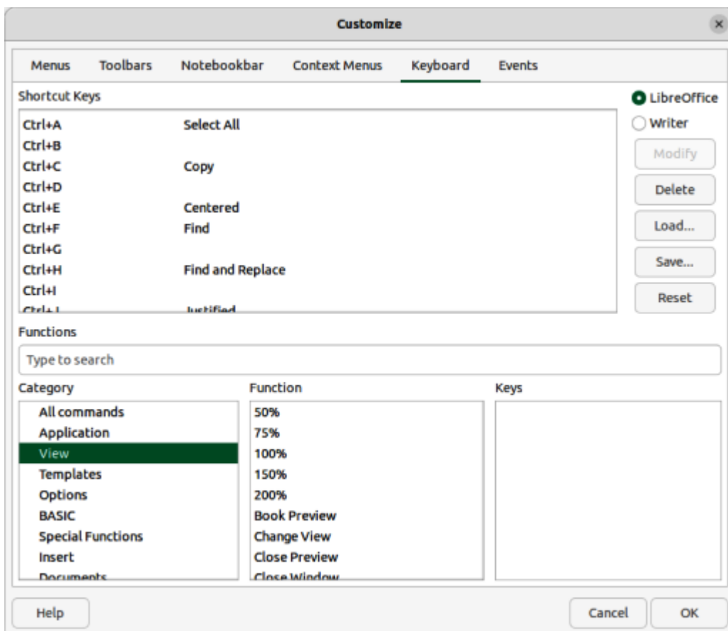
Figure 408: Customize dialog — Keyboard page for Linux/Windows
