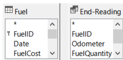
Figure 273: Tables in this query
