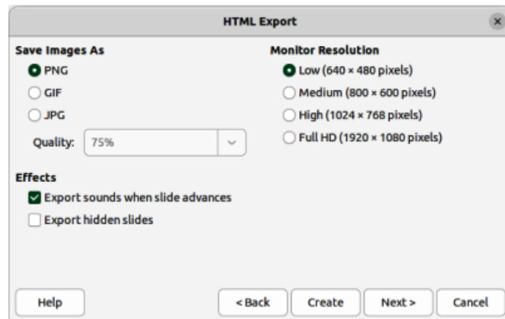
Figure 322: HTML Export dialog — Save images as page
