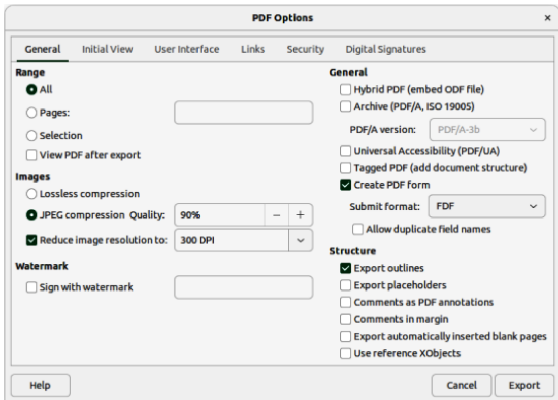
Figure 312: PDF Options dialog — General page
