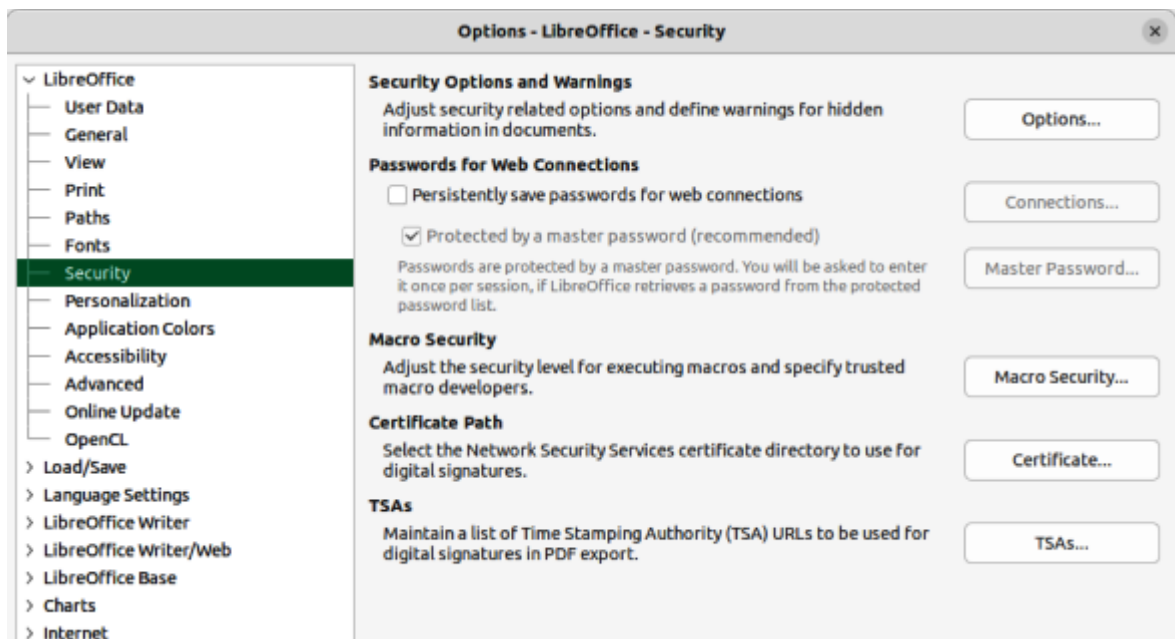
Figure 376: Options LibreOffice dialog — Security page
