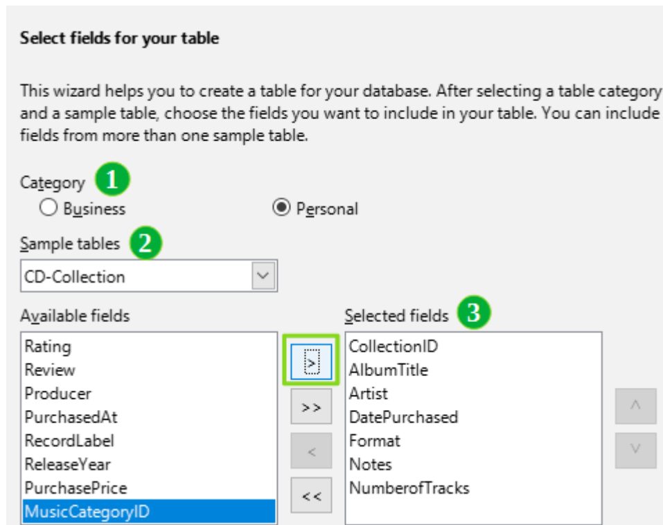
Figure 233: Selecting fields from the Personal category
