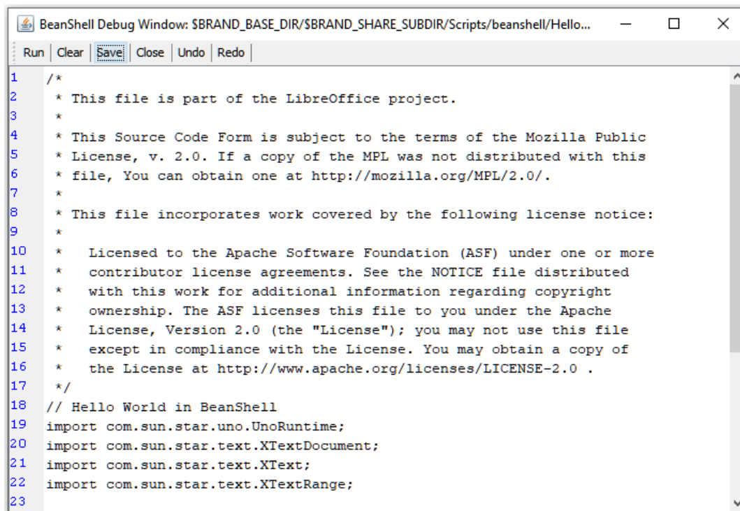
Figure 367: BeanShell Debug Window
