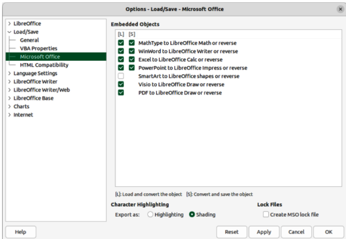
Figure 384: Options Load/Save dialog — Microsoft Office page
