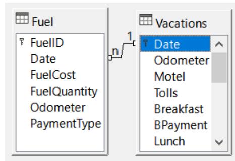
Figure 241: Designation for a 1:n relationship
