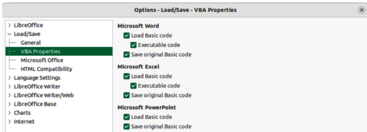
Figure 383: Options Load/Save dialog — VBA Properties page
