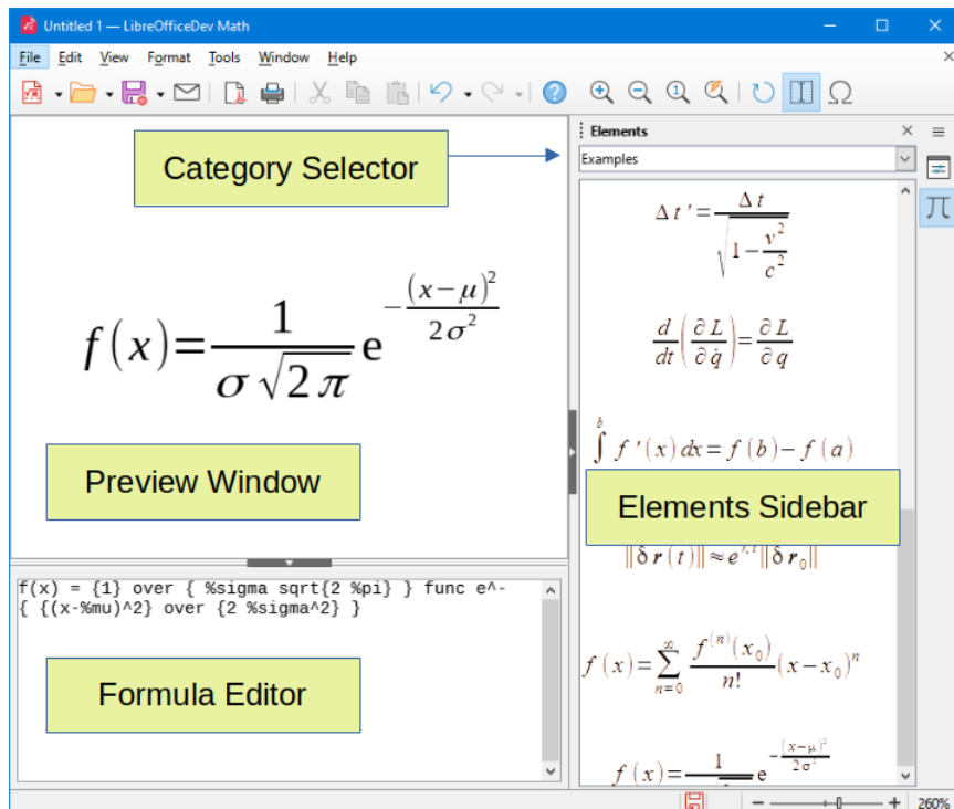
Figure 293: LibreOffice Math window parts
