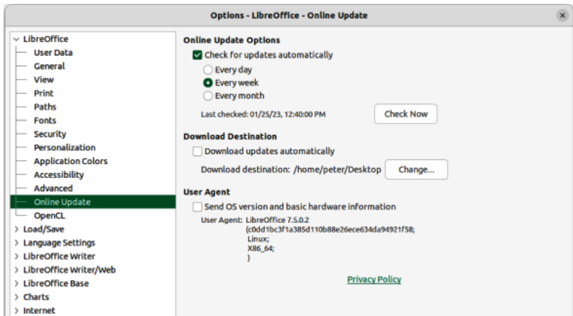
Figure 381: Options LibreOffice dialog — Online Update page
