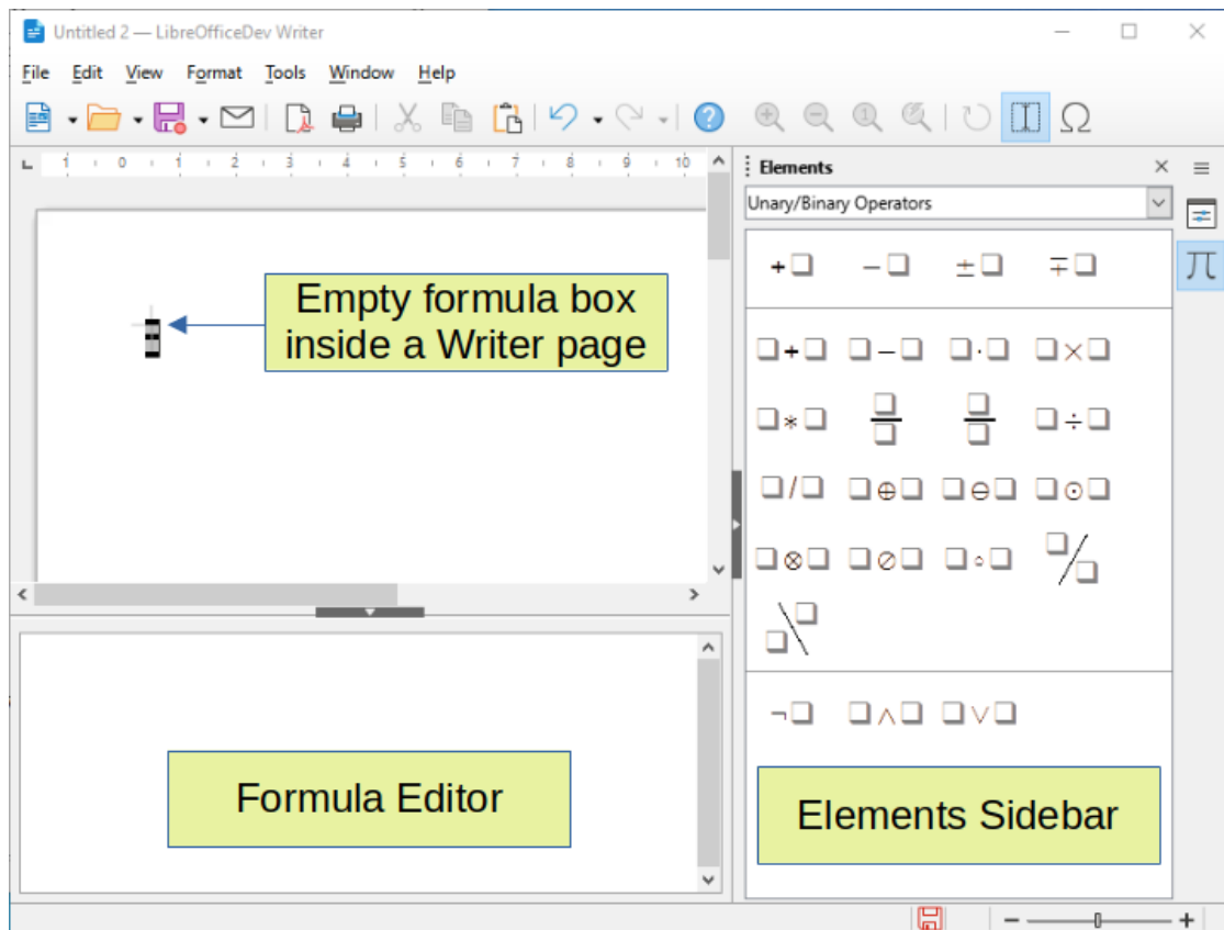
Figure 295: Empty formula in a Writer document
