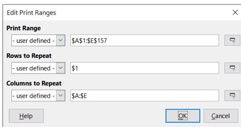
Figure 93: Edit Print Ranges dialog
