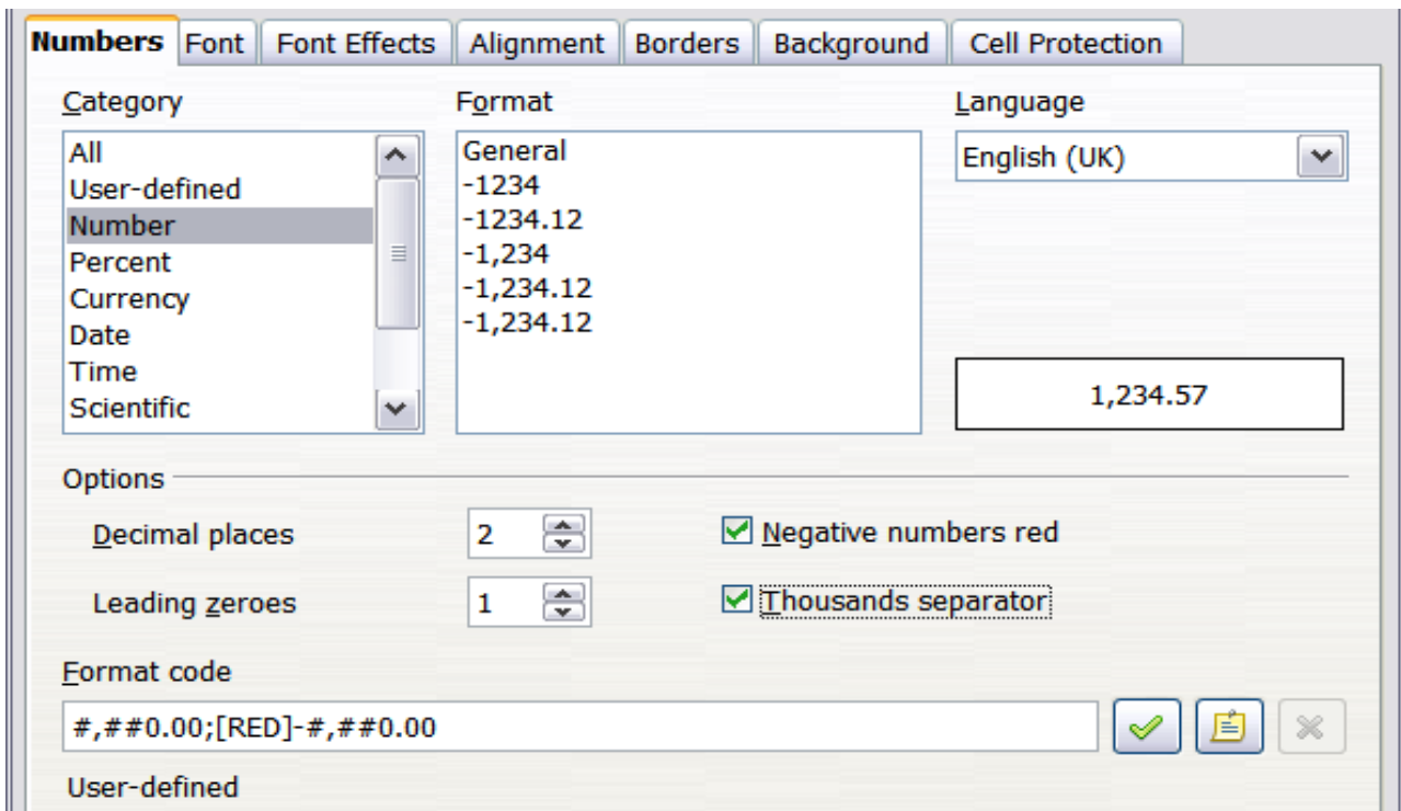
Figure 36: Format Cells > Numbers
