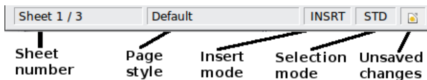
Figure 5: Left end of Calc status bar
