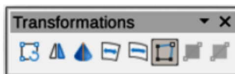
Figure 145: Transformations toolbar
