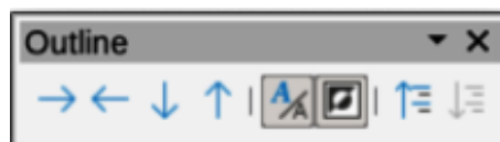
Figure 16: Outline toolbar
