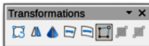
Figure 191: Transformations toolbar
