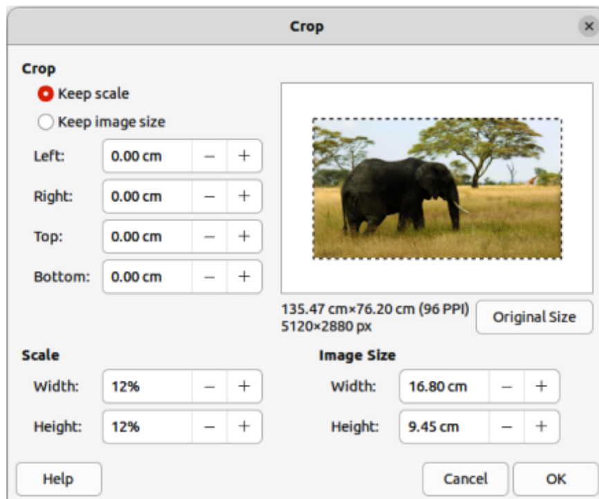
Figure 117: Crop dialog
