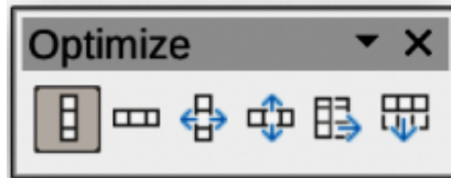
Figure 89: Optimize sub-toolbar
