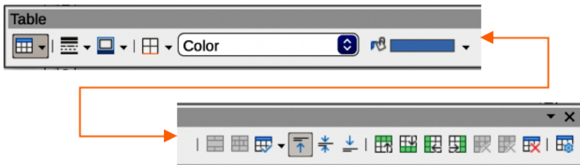
Figure 84: Table toolbar
