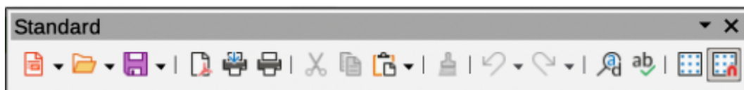
Figure 279: Standard toolbar
