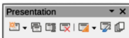
Figure 21: Presentation toolbar
