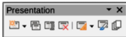
Figure 351: Presentation toolbar
