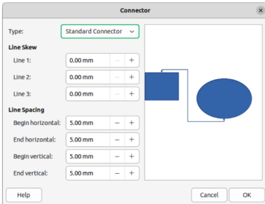
Figure 161: Connector dialog
