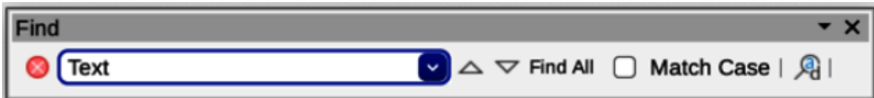
Figure 336: Find toolbar
