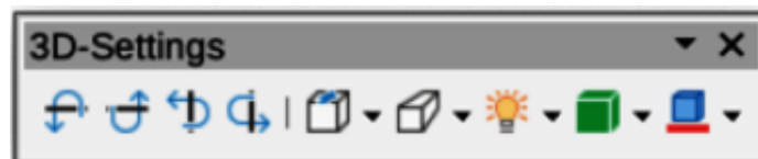
Figure 330: 3D-Settings toolbar
