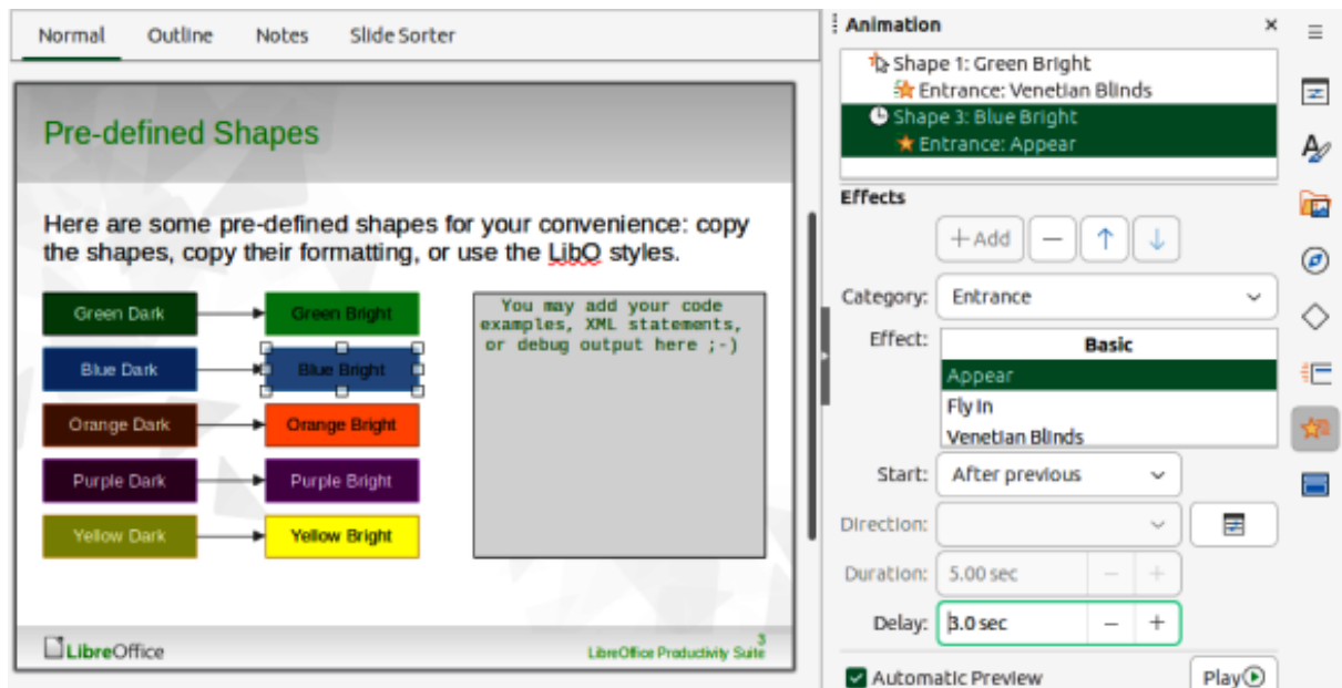
Figure 266: Example animation
