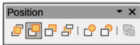
Figure 133: Position sub-toolbar
