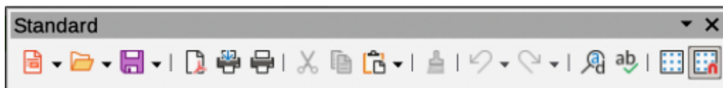
Figure 354: Standard toolbar
