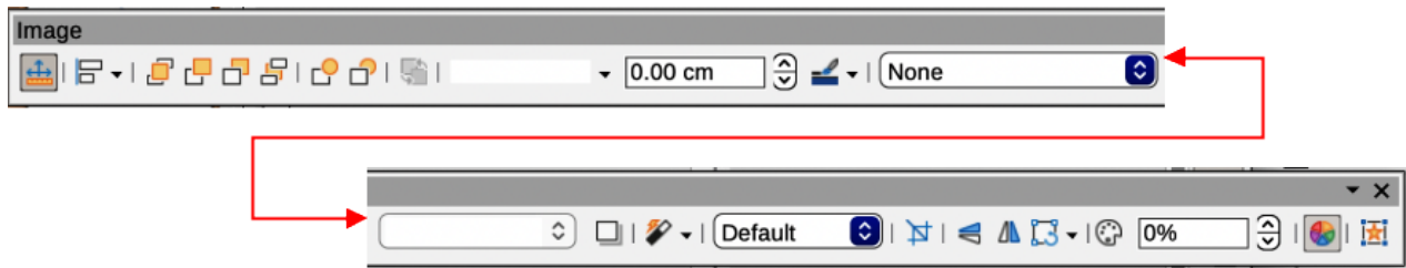
Figure 107: Image toolbar
