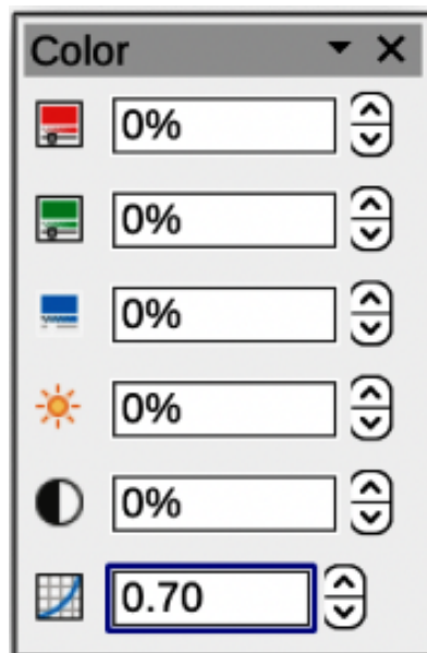
Figure 111: Color sub-toolbar
