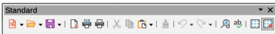
Figure 11: Standard toolbar
