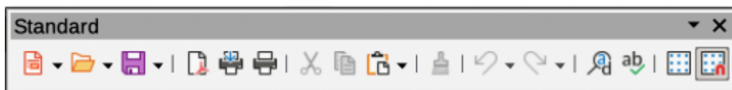
Figure 50: Standard toolbar
