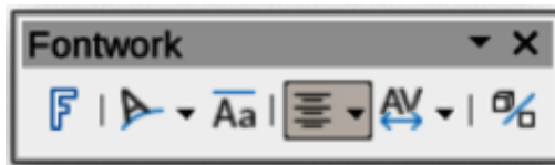
Figure 168: Fontwork toolbar
