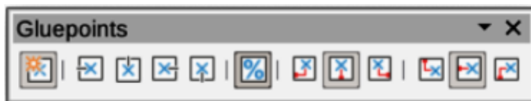
Figure 341: Gluepoints toolbar
