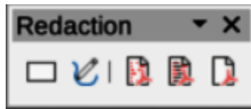
Figure 296: Redaction toolbar
