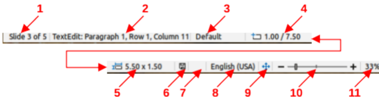
Figure 9: Status Bar
