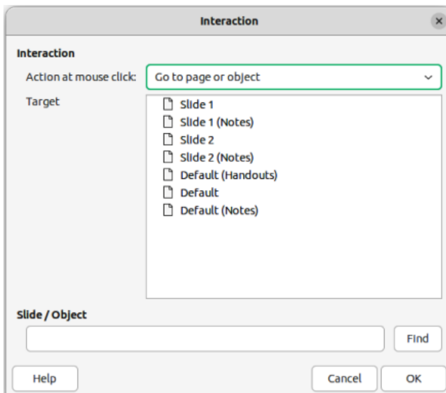
Figure 165: Interaction dialog
