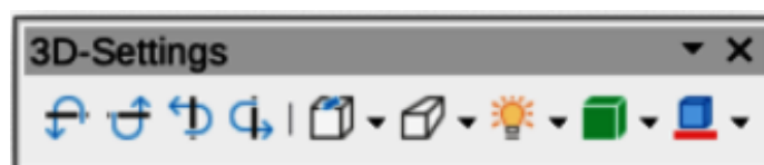
Figure 164: 3D-Settings toolbar
