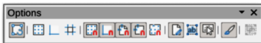
Figure 302: Options toolbar
