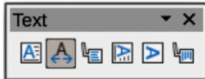
Figure 81: Text toolbar
