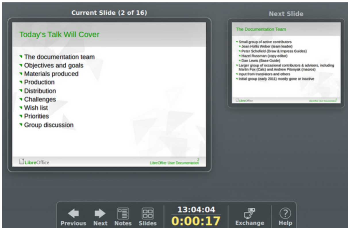
Figure 25: Presenter Console
