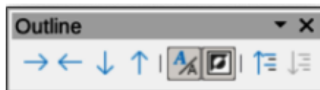
Figure 237: Outline toolbar
