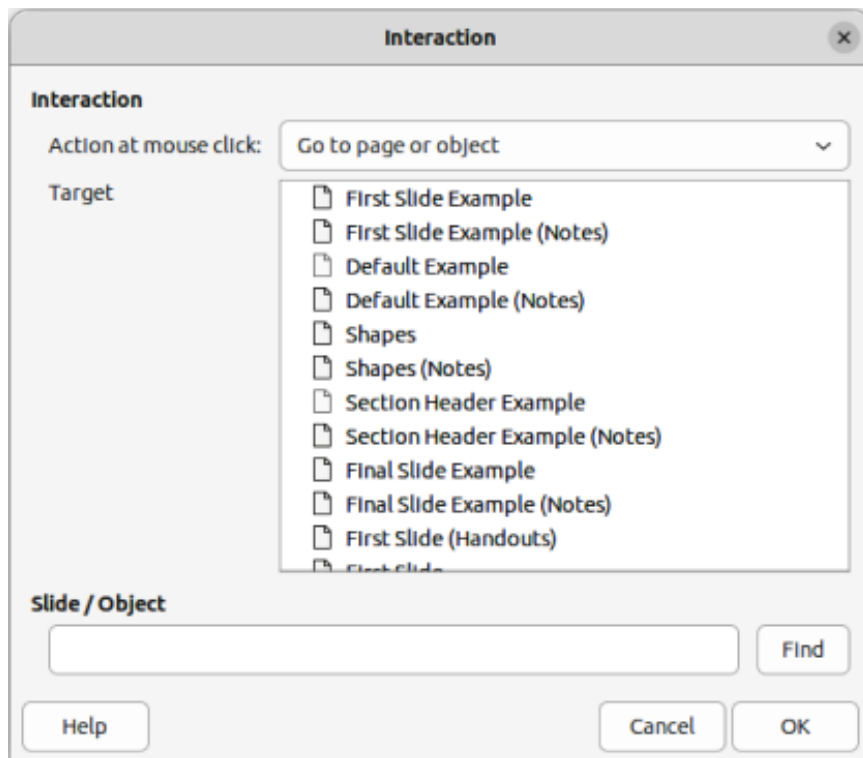
Figure 267: Interaction dialog
