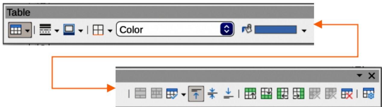
Figure 357: Table toolbar
