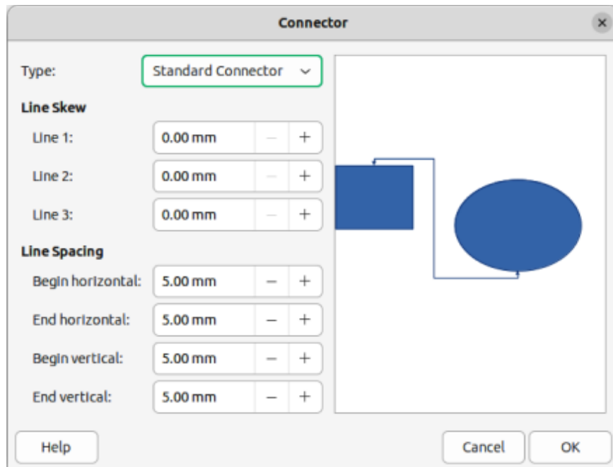
Figure 204: Connector dialog
