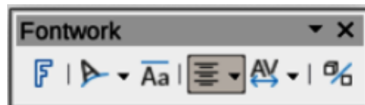
Figure 337: Fontwork toolbar
