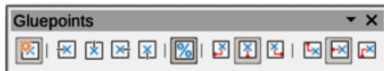
Figure 162: Gluepoints toolbar
