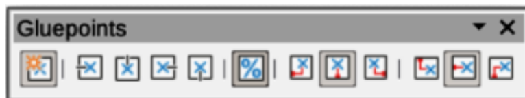
Figure 136: Gluepoints toolbar
