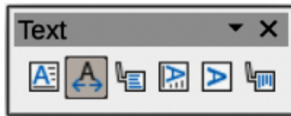
Figure 358: Text toolbar
