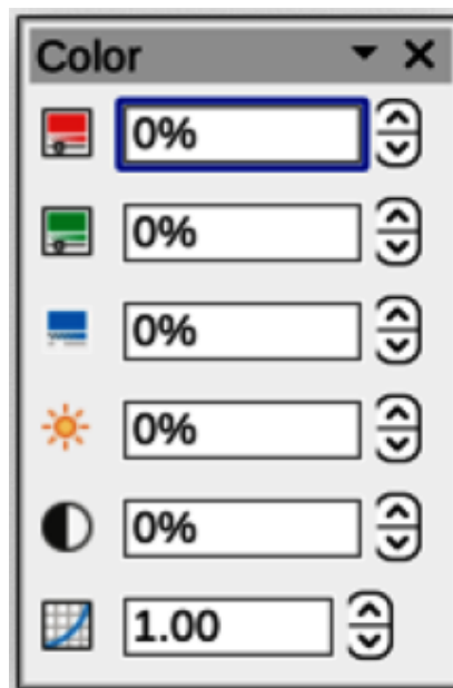
Figure 367: Color sub-toolbar
