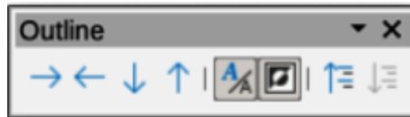
Figure 350: Outline toolbar
