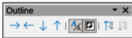
Figure 75: Outline toolbar
