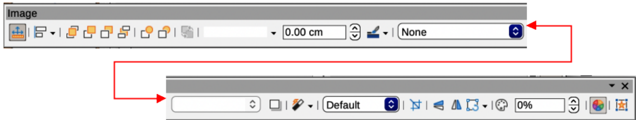
Figure 342: Image toolbar
