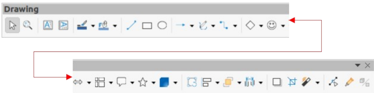
Figure 6: Drawing toolbar
