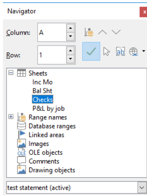
Figure 10: Navigator dialog
