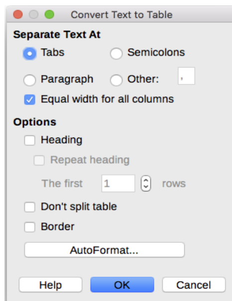
Figure 3: Dialog for the text to table conversion
