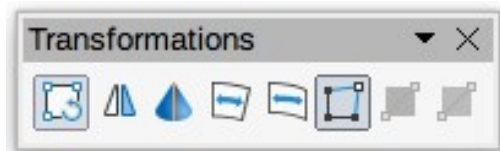
Figure 15: Transformations toolbar
