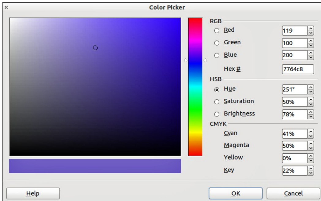
Figure 9: Editing colors
