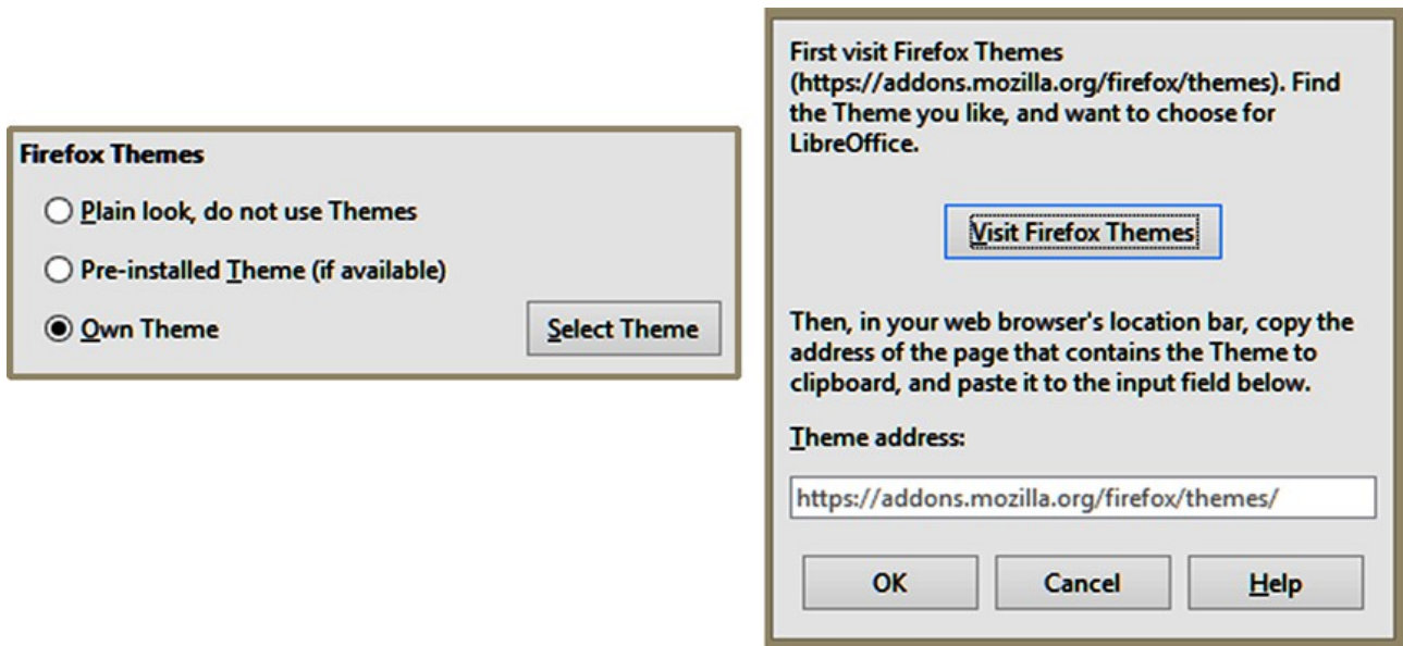
Figure 14: Personalization dialogs
