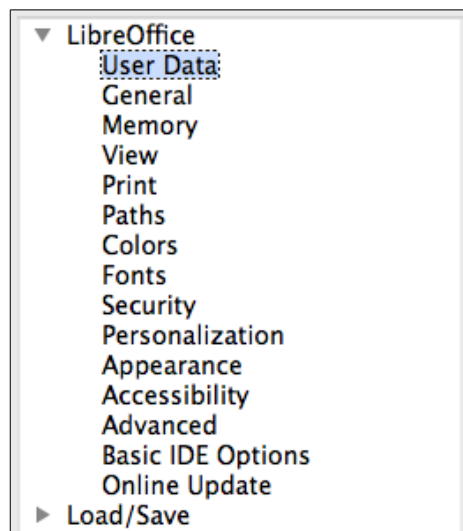
Figure 1: LibreOffice options
