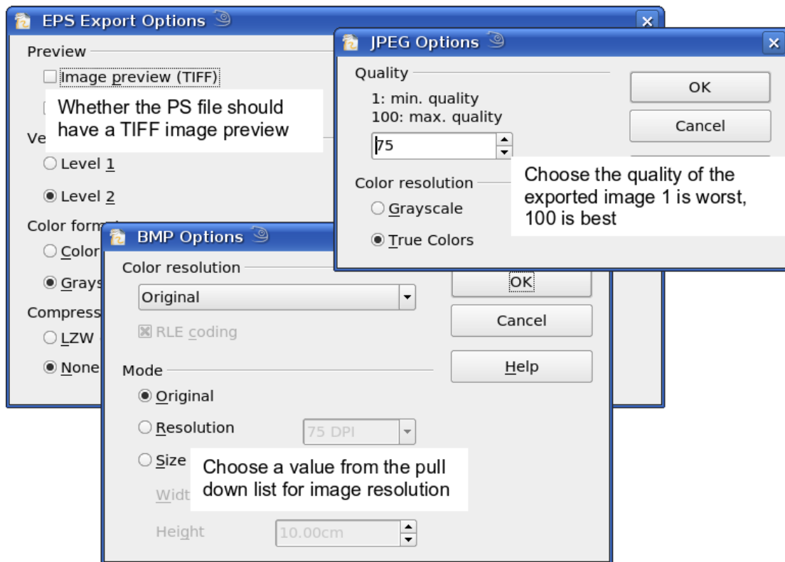
Figure 122: Adjusting format specific properties prior to export
