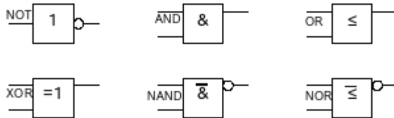
Figure 216: Logic Symbol library
