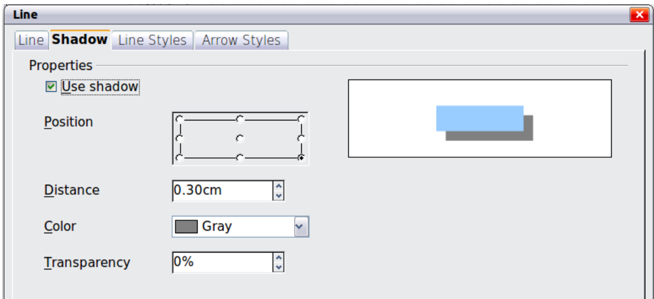
Figure 75: Shadow page of Line dialog
