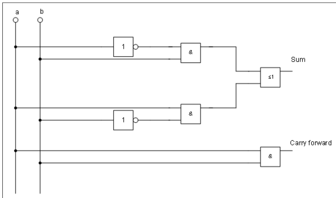
Figure 223: Half adder drawn using logic symbol building blocks
