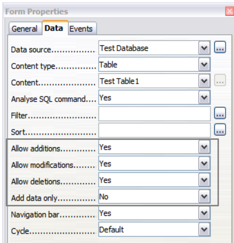
Figure 436: Data Properties of a form
