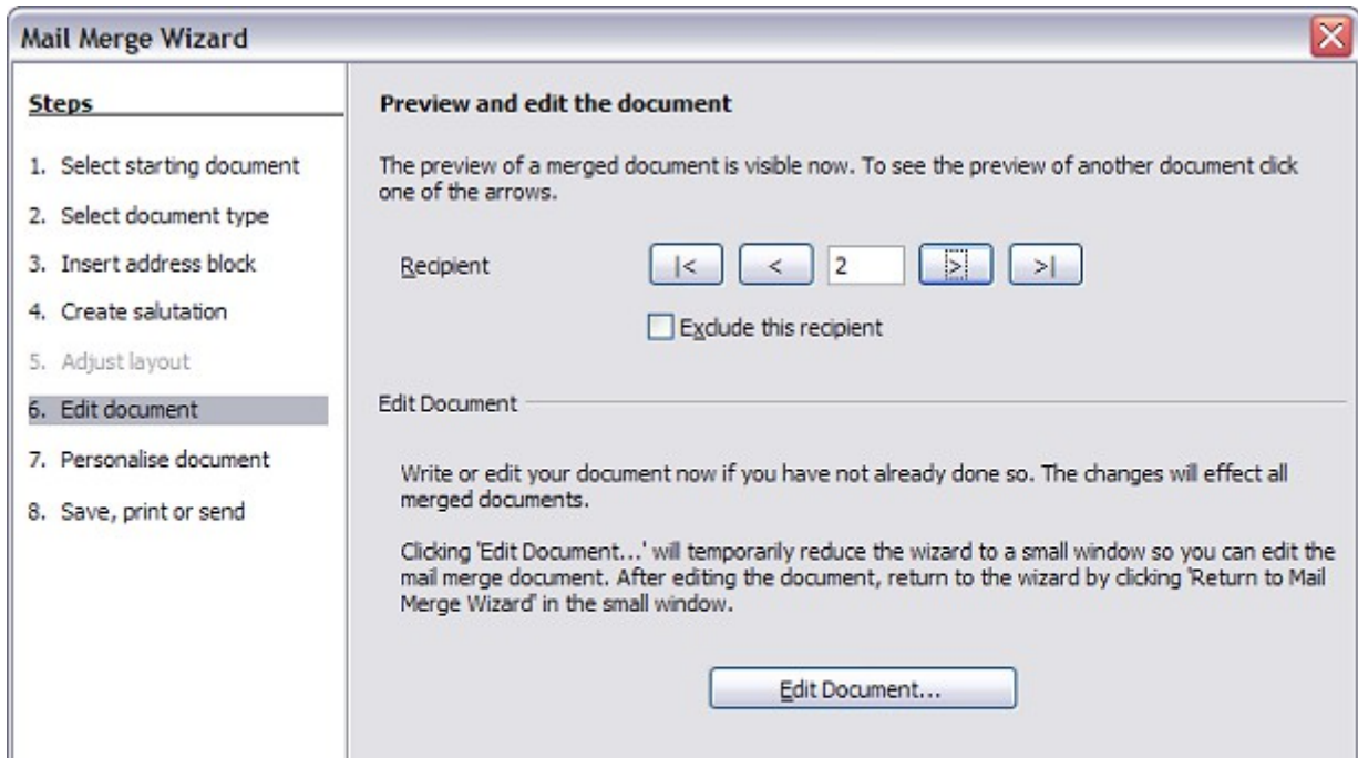
Figure 330: Edit document
