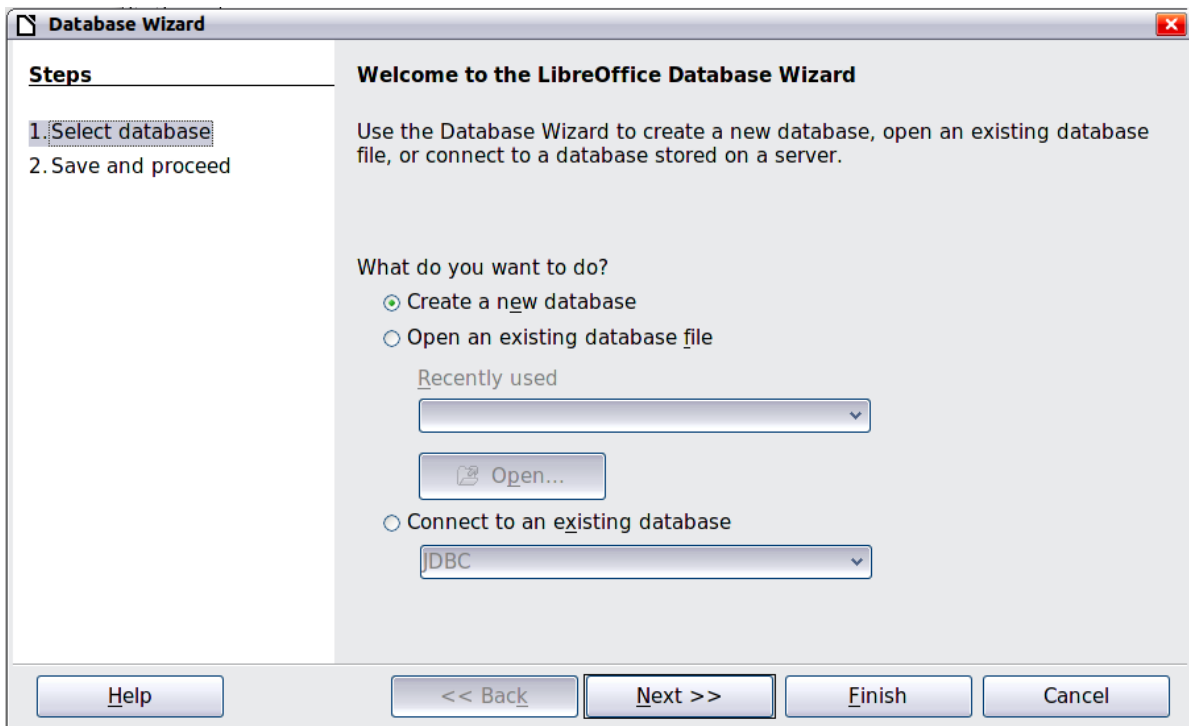
Figure 426: Database Wizard
