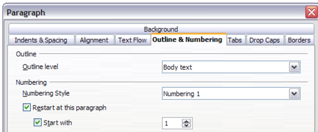
Figure 198: Restarting numbering
