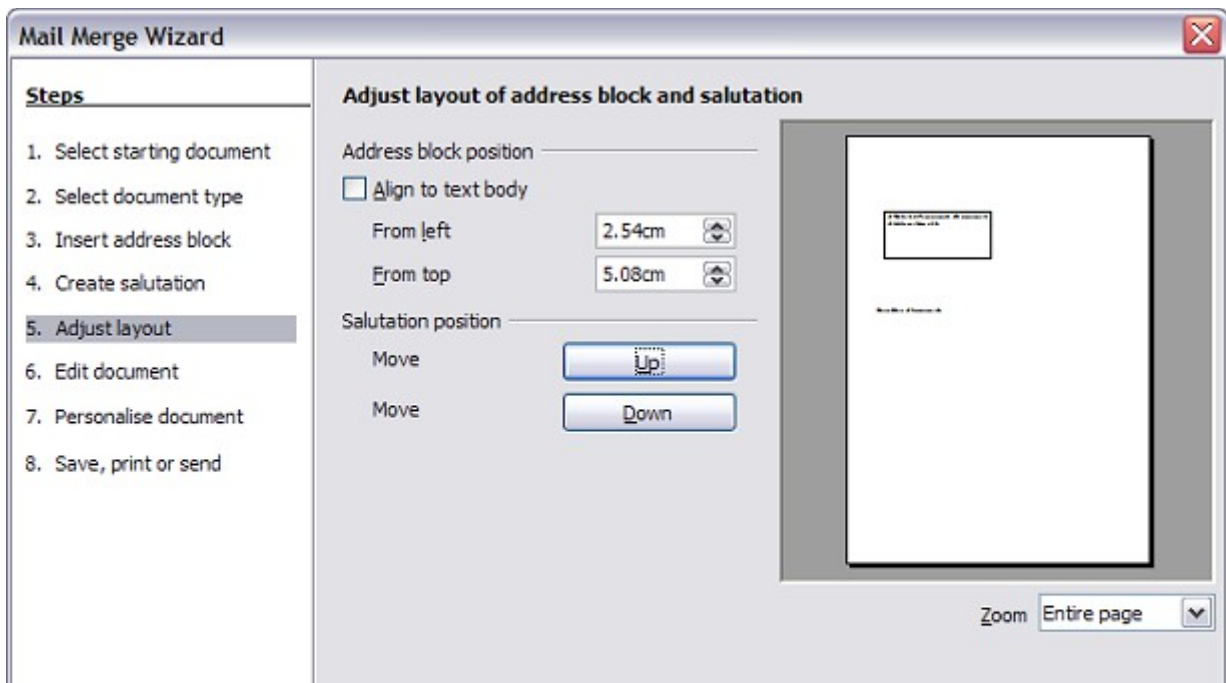
Figure 329: Adjust layout
