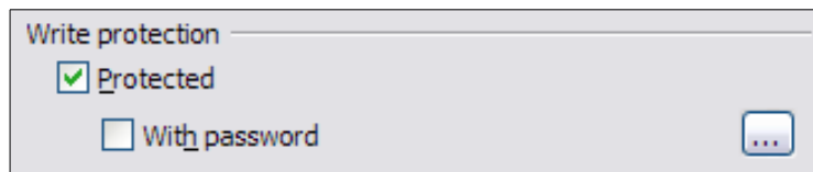
Figure 130: Write-protecting sections
