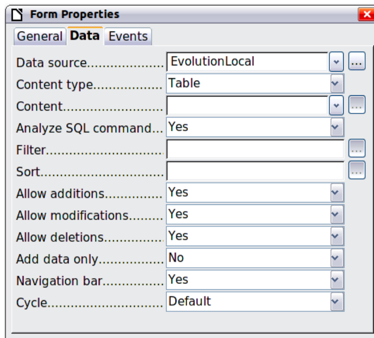
Figure 431: Form properties, connecting to a data source
