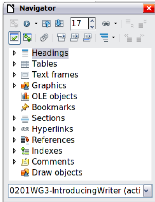
Figure 21. The Navigator
