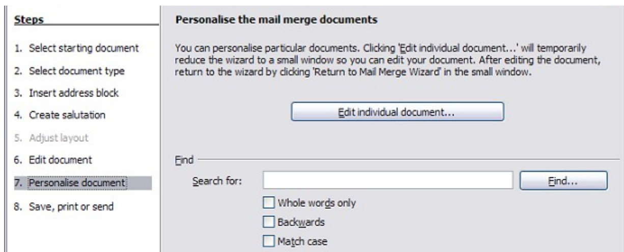
Figure 333: Personalize document
