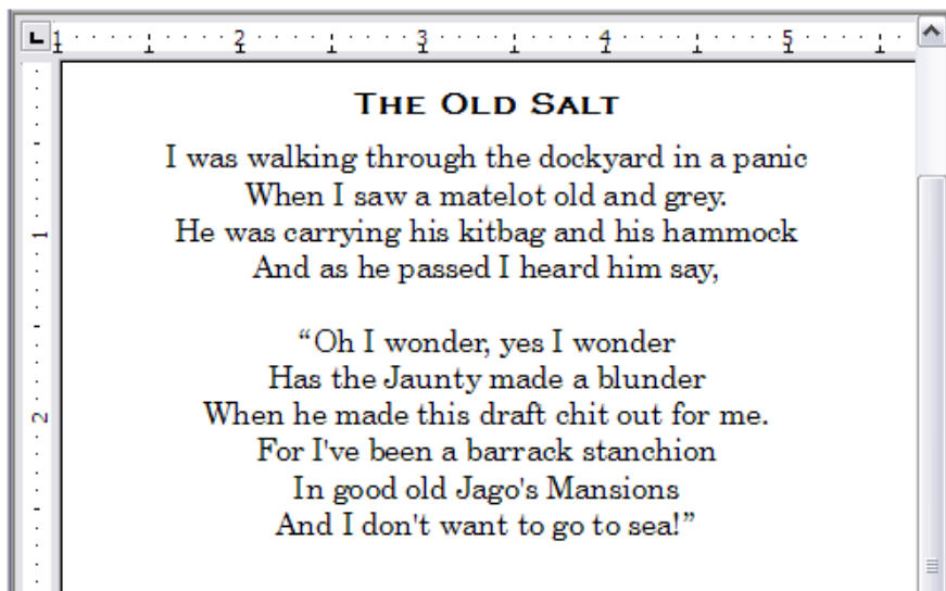
Figure 209: Sample poem
