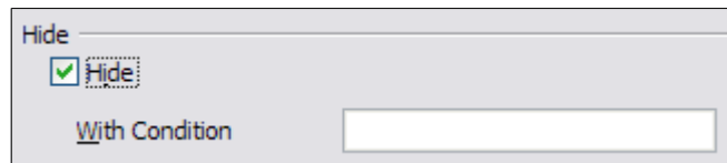
Figure 132: Hiding sections
