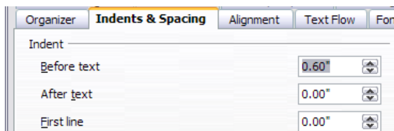
Figure 204: Set indentation
