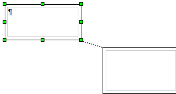
Figure 120: Linked frames
