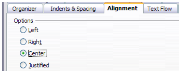
Figure 202: Center Heading 1
