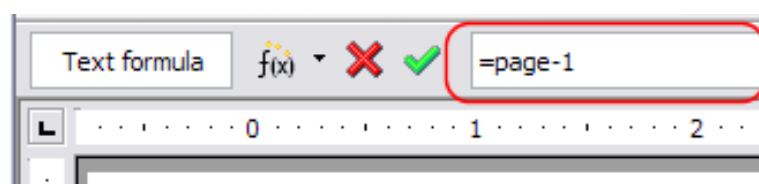
Figure 154: Formula bar
