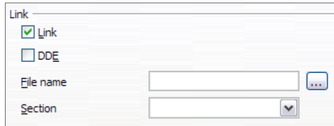
Figure 129: Linking sections
