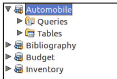
Figure 28: Databases
