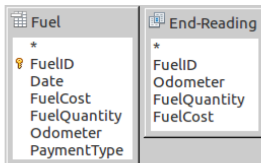
Figure 46: Tables in this query
