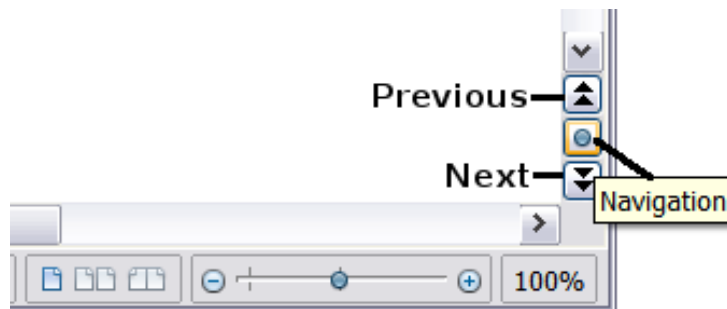
Figure 6: Navigation icons
