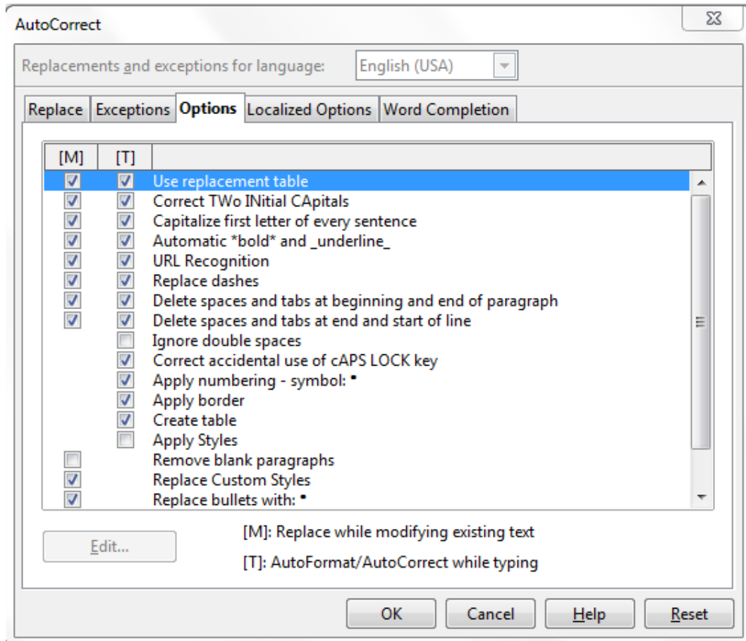
Figure 28: The AutoCorrect dialog in Writer, showing the five tabs and some of the choices
