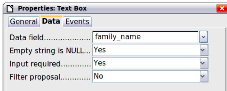
Figure 425: Form control properties, Data tab
