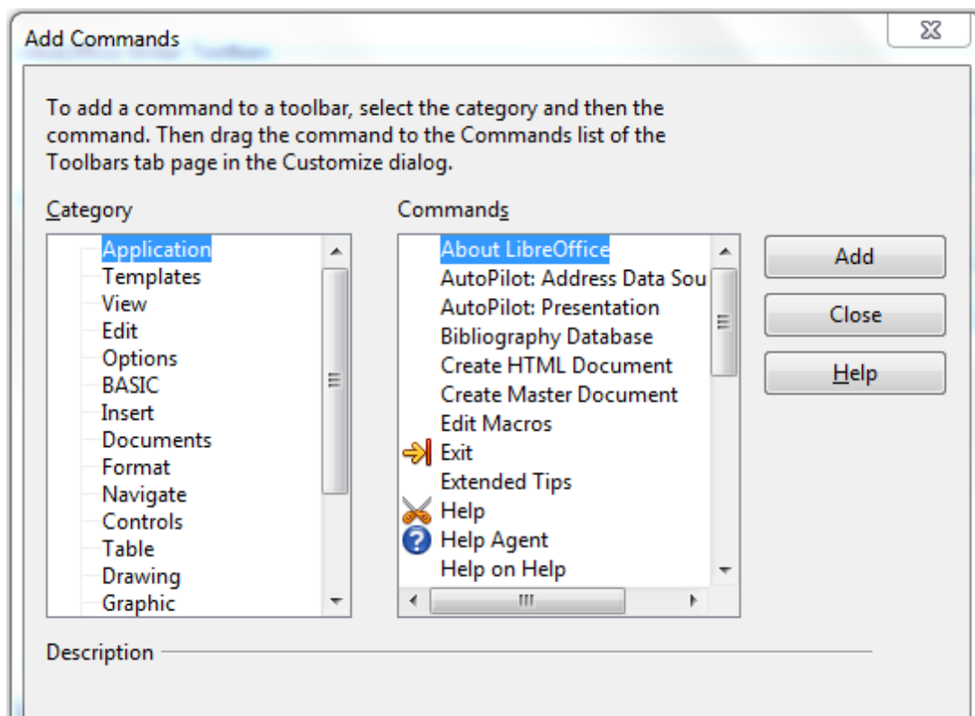
Figure 432: Adding a command to a menu
