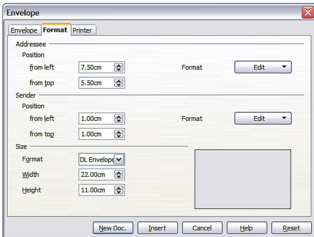
Figure 313: Envelope formatting dialog box
