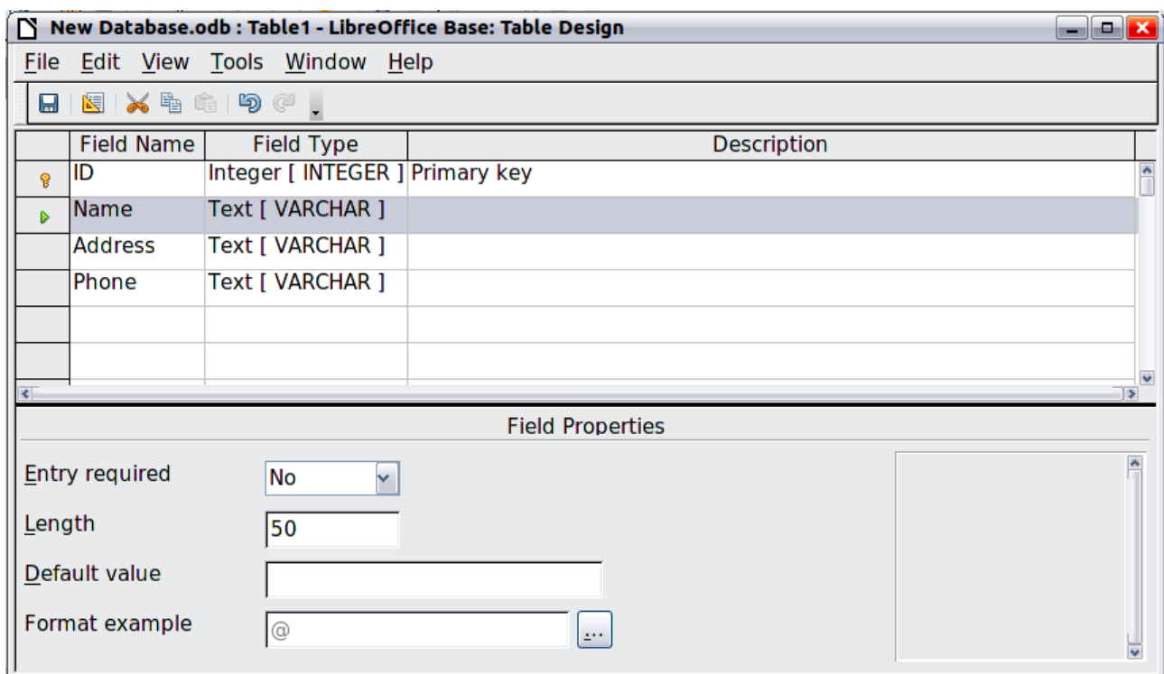
Figure 422: Database table design
