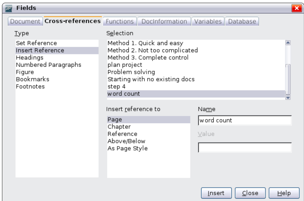
Figure 376. Fields dialog box showing manual entry of field name
