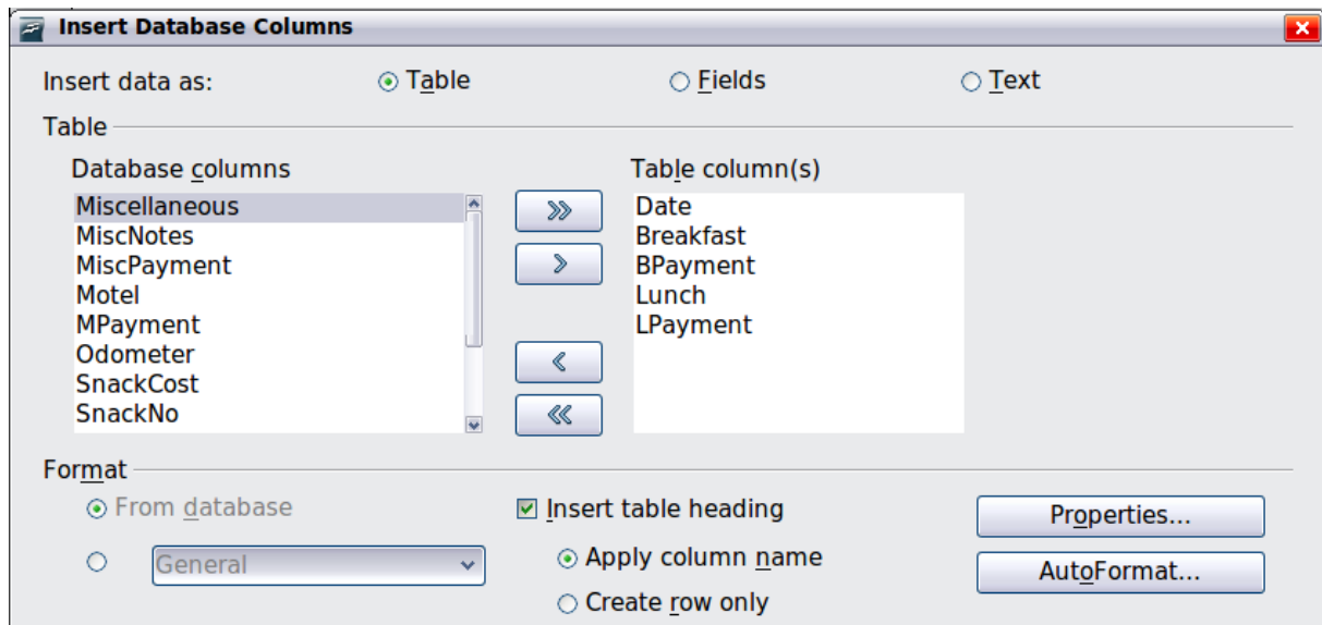
Figure 32: Insert Database Columns dialog
