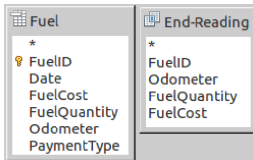
Figure 45: Tables in this query
