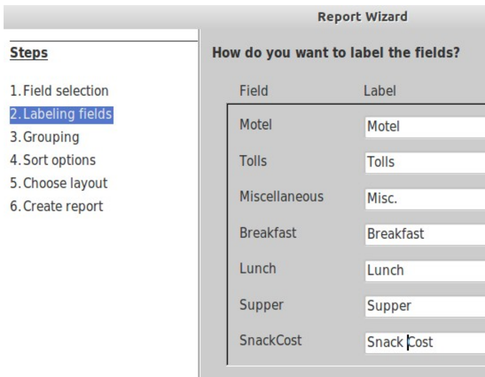
Figure 56: Giving aliases to fields
