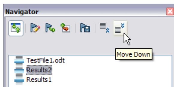
Figure 4: Moving subdocuments
