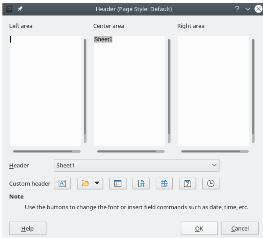
Figure 210: Header dialog
