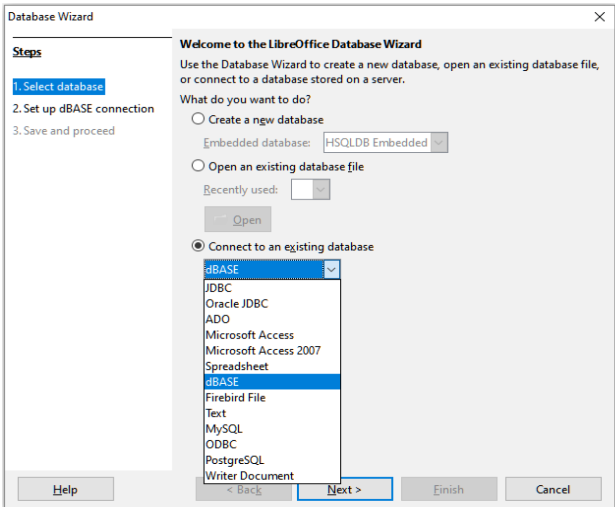
Figure 399: Database Wizard
