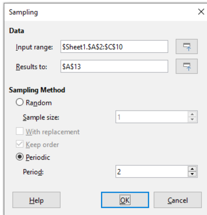
Figure 334: Sampling dialog
