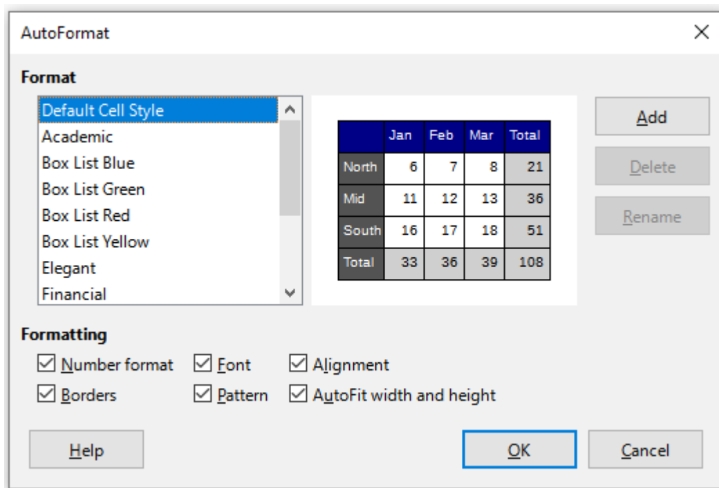
Figure 51: AutoFormat dialog
