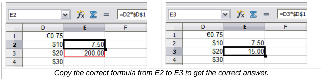
Figure 226: Absolute references
