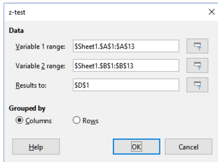
Figure 358: z-test dialog
