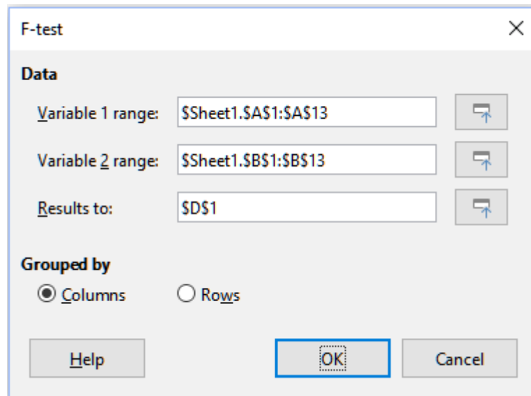
Figure 356: F-test dialog
