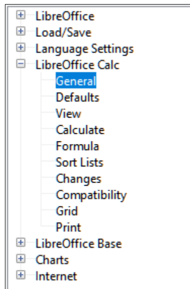
Figure 477: Calc options
