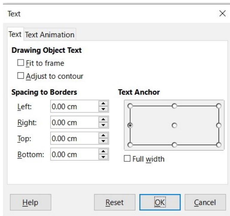
Figure 187: Text dialog
