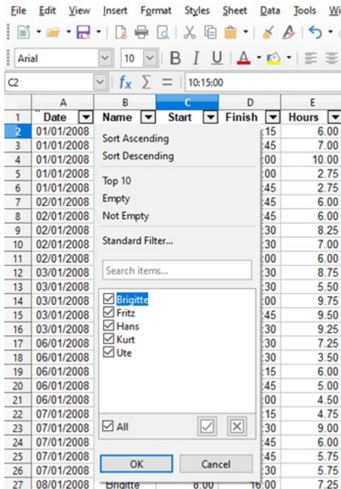
Figure 66: AutoFilter example
