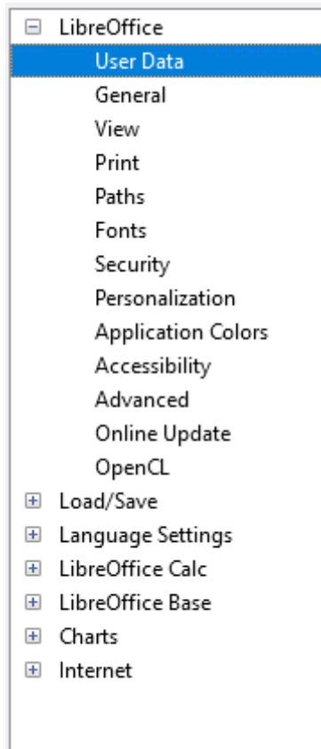
Figure 469: LibreOffice options
