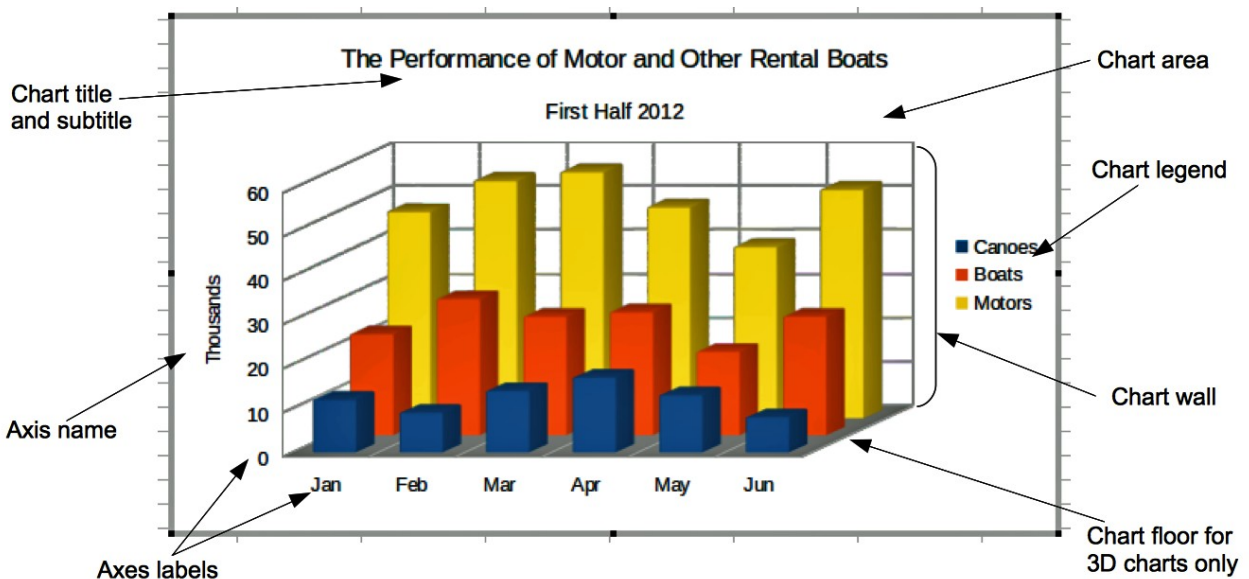
Figure 79: Chart elements
