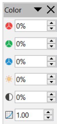
Figure 185: Color toolbar
