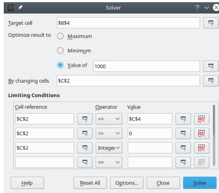
Figure 329: Solver dialog
