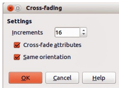
Figure 46: Cross-fading dialog
