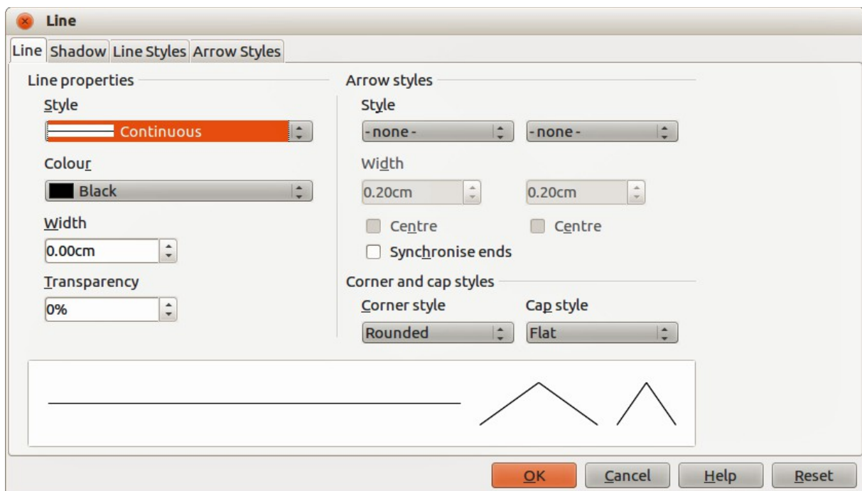
Figure 14: Line dialog
