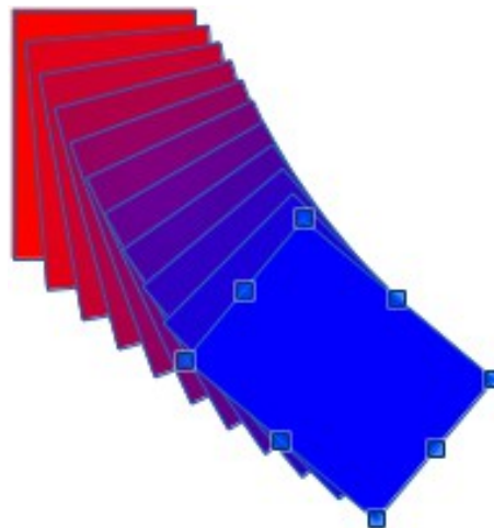
Figure 45: Duplication result
