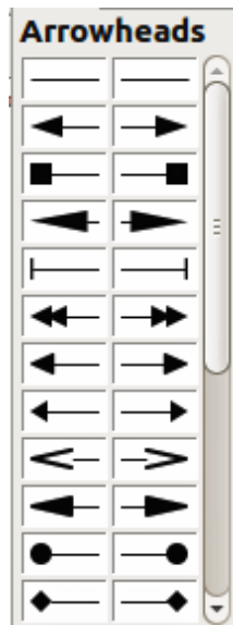
Figure 39: Arrowheads menu
