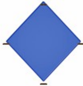
Figure 18: Glue points
