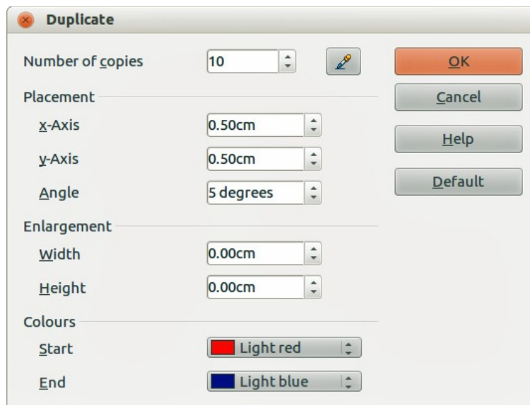
Figure 44: Duplicate dialog
