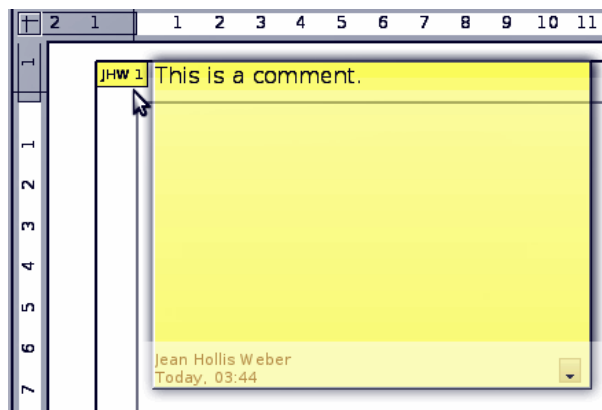
Figure 48: Inserting comments
