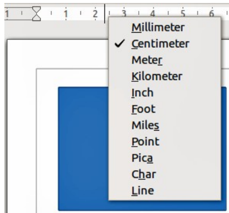
Figure 3: Ruler units
