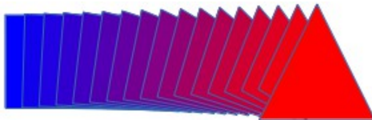
Figure 47: Cross-fading result
