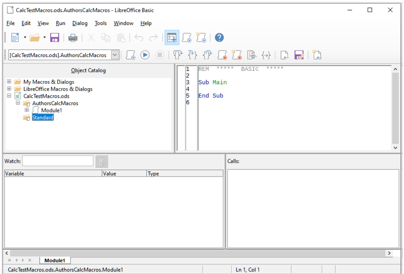
Figure 12: LibreOffice Basic Integrated Development Environment
