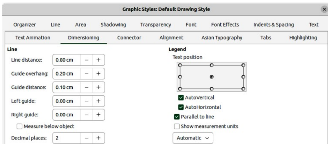
Figure 289: Graphic Styles dialog — Dimensioning page
