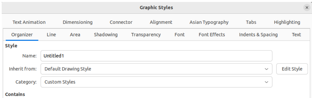
Figure 32: Graphic Styles dialog - Organizer page
