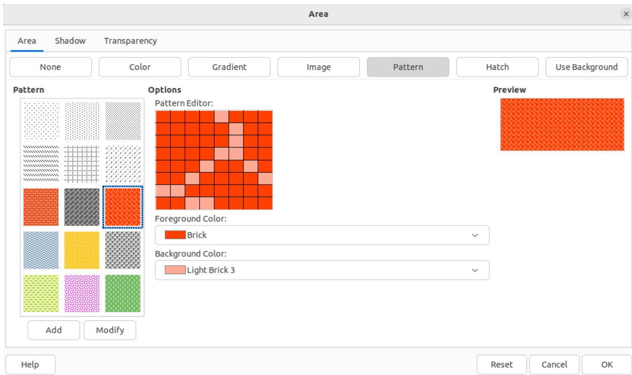
Figure 20: Area dialog - Pattern page
