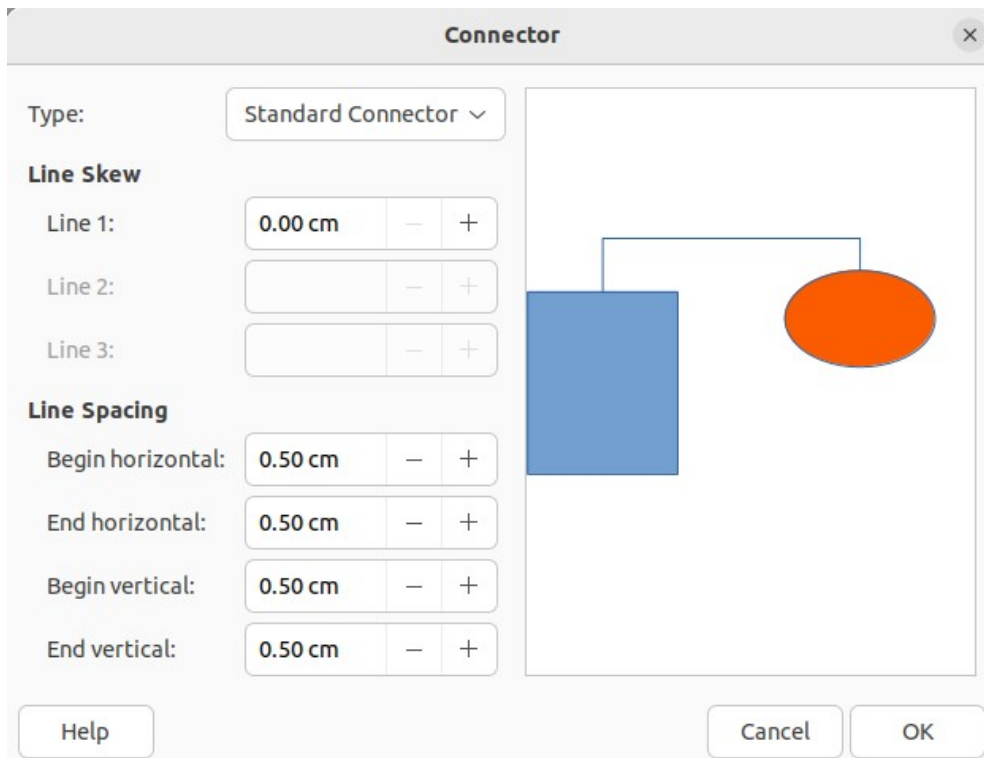
Figure 30: Connector dialog
