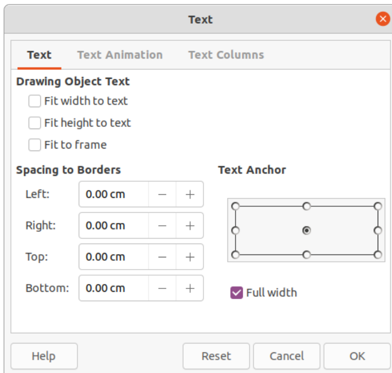
Figure 27: Text dialog - Text page
