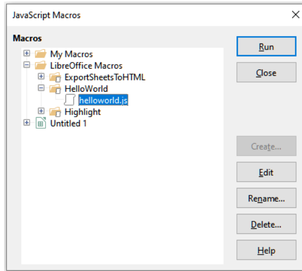
Figure 24: JavaScript Macros dialog
