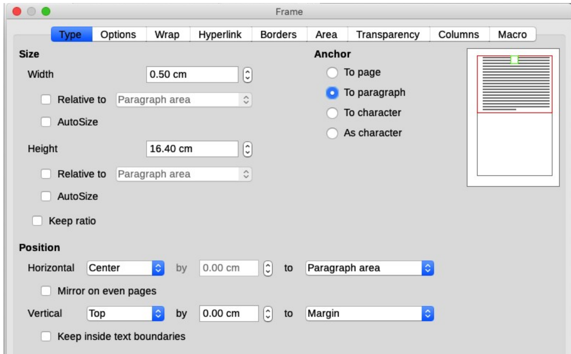
Figure 29: Defining the size and position of the footer frame
