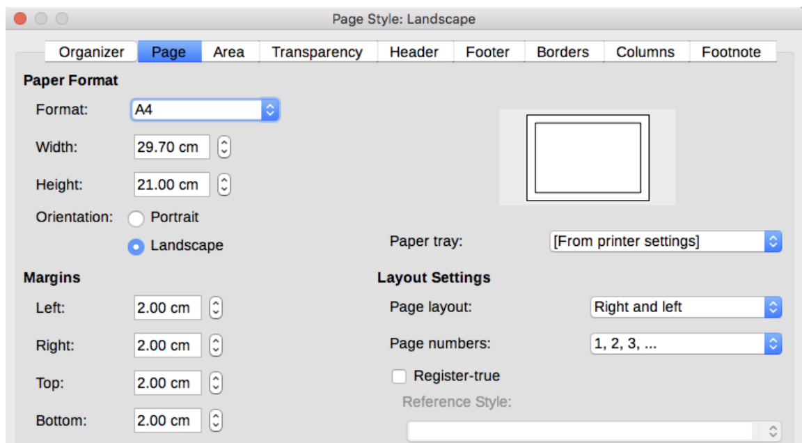
Figure 24: Set orientation and margins for a landscape page
