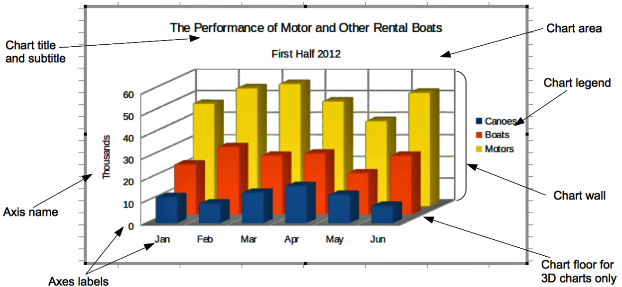
Figure 7: Chart elements
