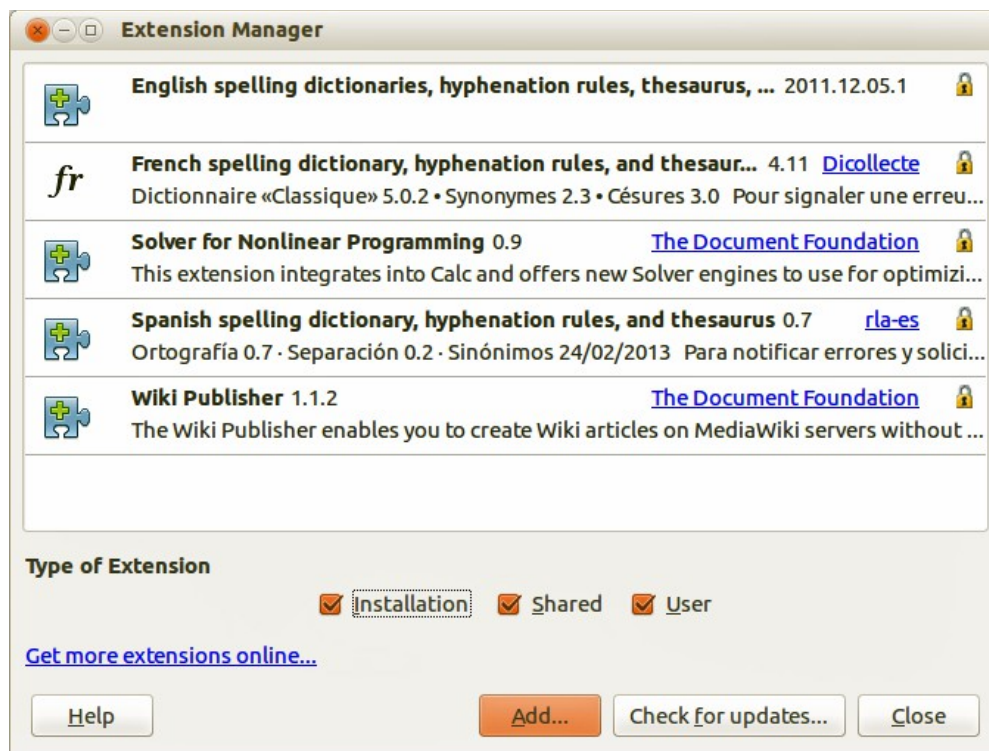
Figure 16: Extension Manager
