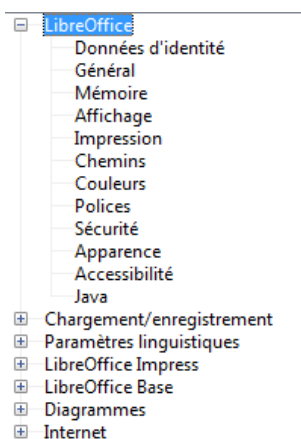
Figure 1 : Options LibreOffice
