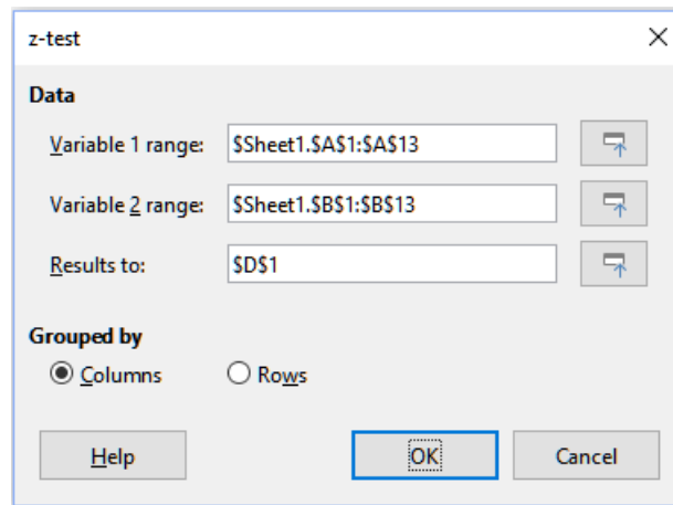
Figure 58: z-test dialog
