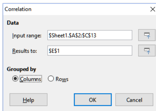
Figure 41: Correlation dialog
