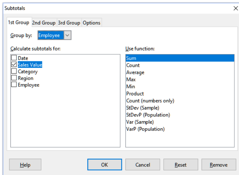
Figure 9: Subtotals dialog
