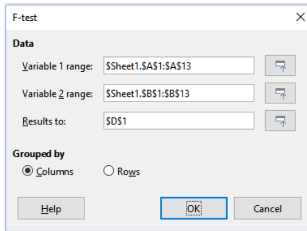
Figure 56: F-test dialog
