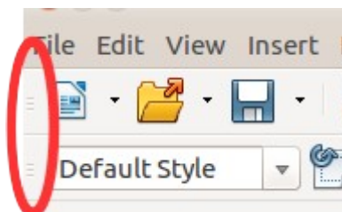
Figure 3: Toolbar handles
