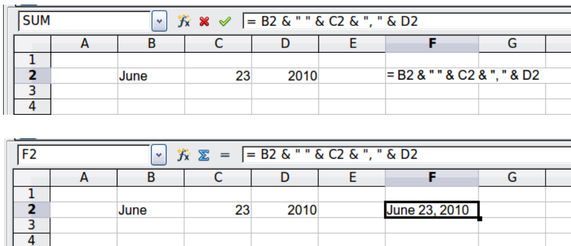
Figure 3: Text concatenation
